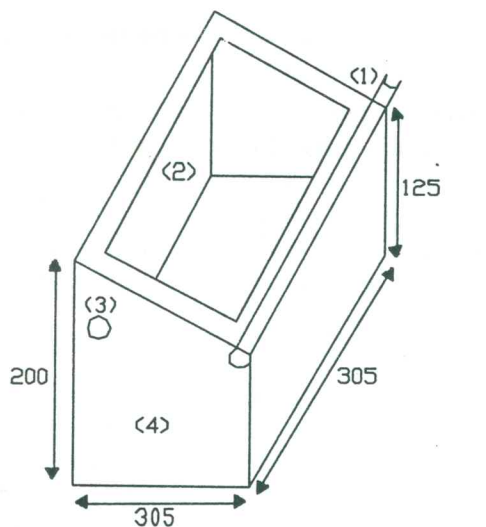
(1) D.I. water collection pipe (2) Glass (3) Acid zinc wash water (4) P V C sheet
