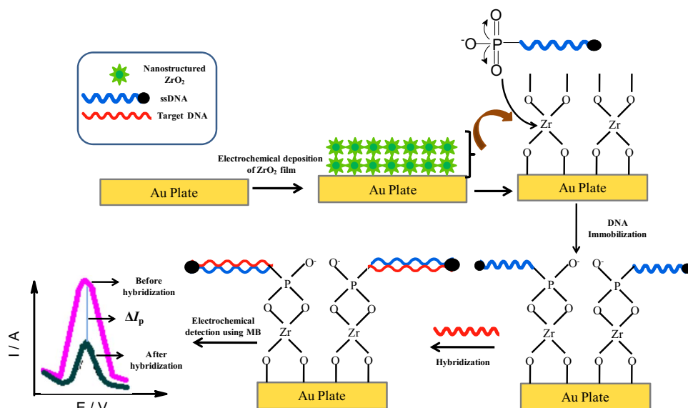
FIG. 1. (Color online) Proposed schematic for the fabrication of nanoZrO 2 /Au based DNA biosensor.
