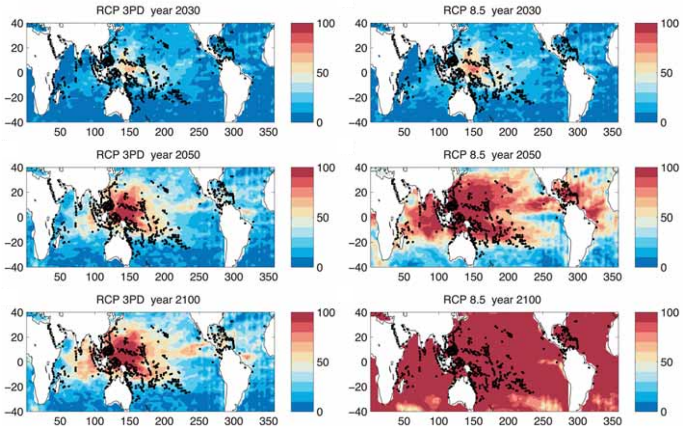
Figure 4.11: Projected impact of climate change on coral systems in South East Asia
