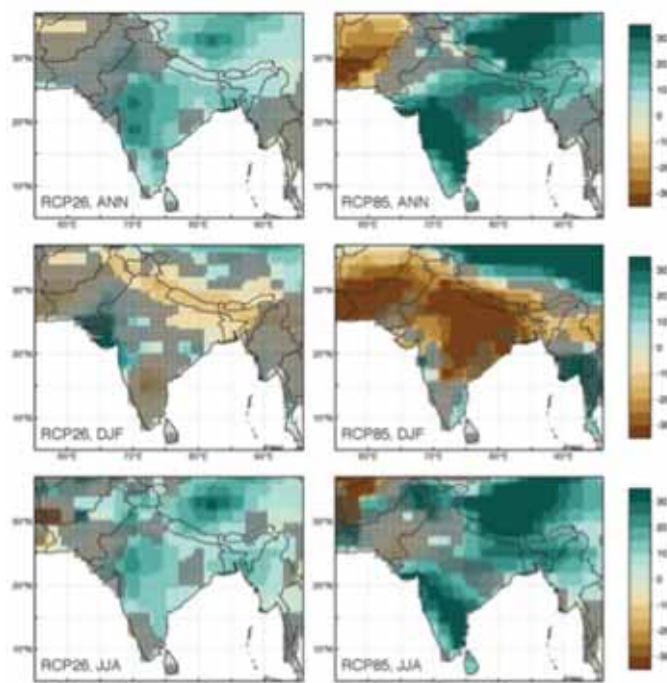
Figure 4 Projected impact of climate change on annual, wet and dry season rainfall in South Asia
