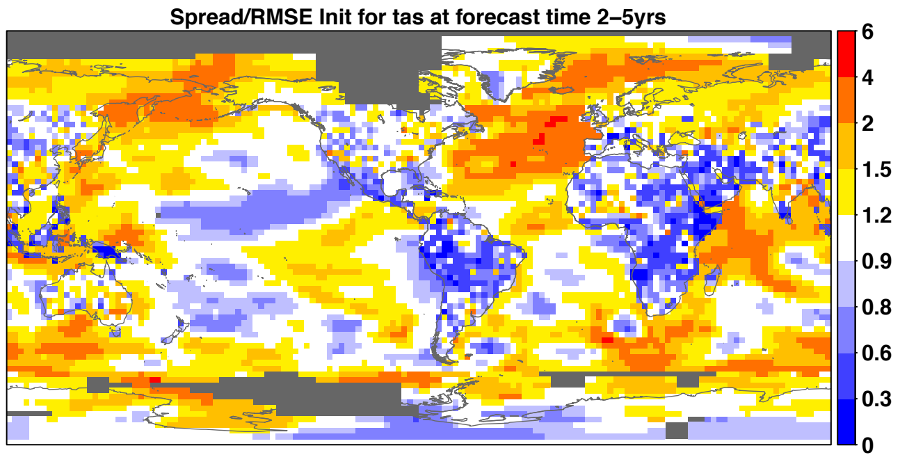
Figure 11.7 | Ratio between the surface temperature spread around the ensemble mean and the root mean square error (RMSE) of the ensemble-mean prediction of Init and Nlnit for the forecast time 2 to 5 years with 5-year interval between start dates over the period 1960–2005. A combination of temperatures from Global Historical Climatology Network/Climate Anomaly Monitoring System (GHCN/CAMS) air temperature over land, Extended Reconstructed Sea Surface Temperature (ERSST) v3b over sea and Goddard Institute of Space Studies Surface Temperature Analysis (GISTEMP) 1200 over the polar areas is used as a reference to compute the RMSE. (Adapted from Doblas-Reyes et al., 2013.)
