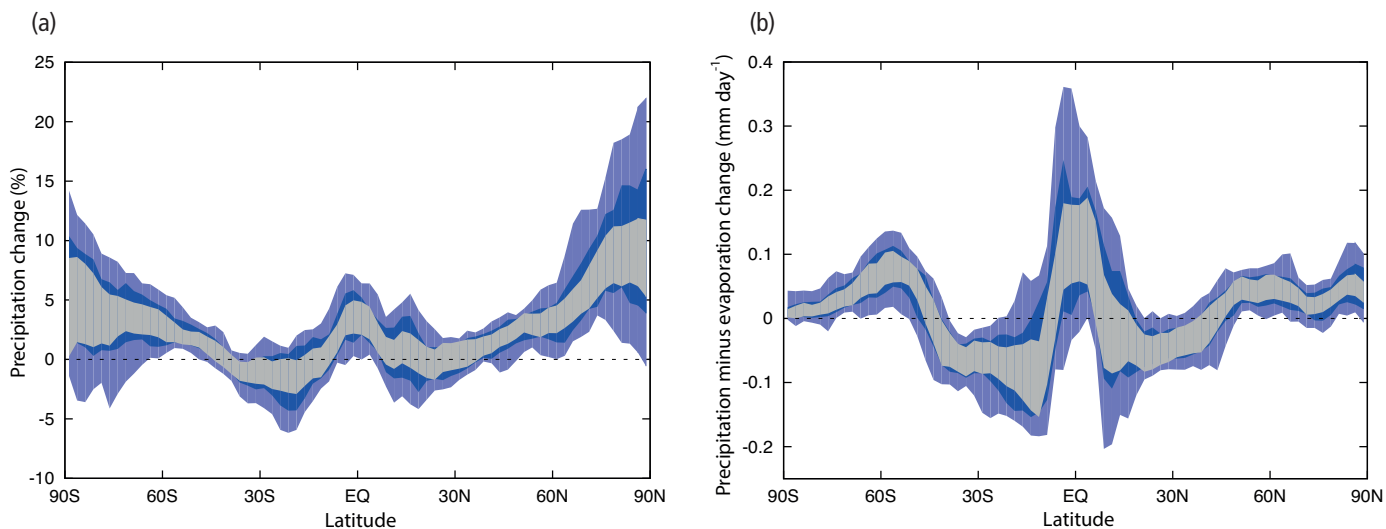
Figure 11.13 | CMIP5 multi-model projections of changes in annual and zonal mean (a) precipitation (%) and (b) precipitation minus evaporation (mm day -1 ) for the period 2016–2035 relative to 1986–2005 under RCP4.5. The light blue denotes the 5 to 95% range, the dark blue the 17 to 83% range of model spread. The grey indicates the 1σ range of natural variability derived from the pre-industrial control runs (see Annex I for details).
