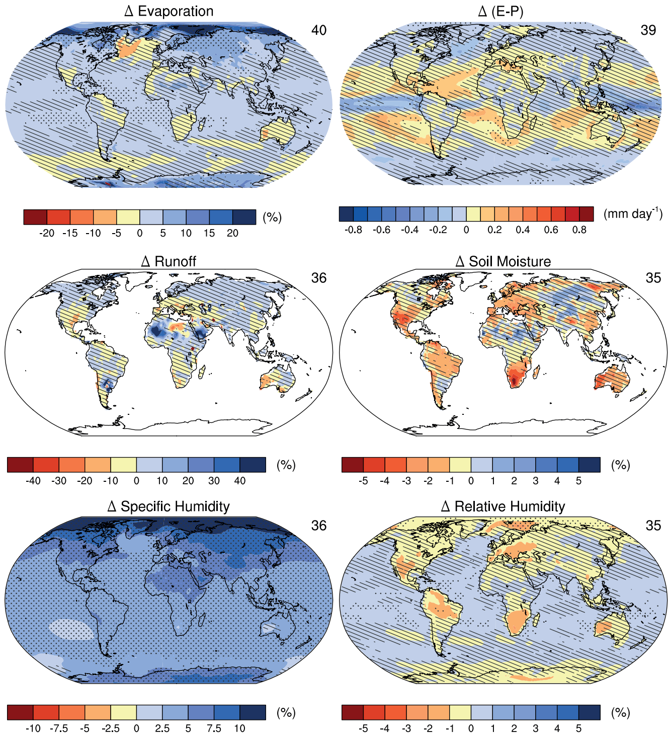
Figure 11.14 | CMIP5 multi-model annual mean projected changes for the period 2016–2035 relative to 1986–2005 under RCP4.5 for: (a) evaporation (%), (b) evaporation minus precipitation ( E - P , \text{mm day}^{-1} ), (c) total runoff (%), (d) soil moisture in the top 10 cm (%), (e) relative change in specific humidity (%), and (f) absolute change in relative humidity (%). The number of CMIP5 models used is indicated in the upper right corner of each panel. Hatching and stippling as in Figure 11.10.
