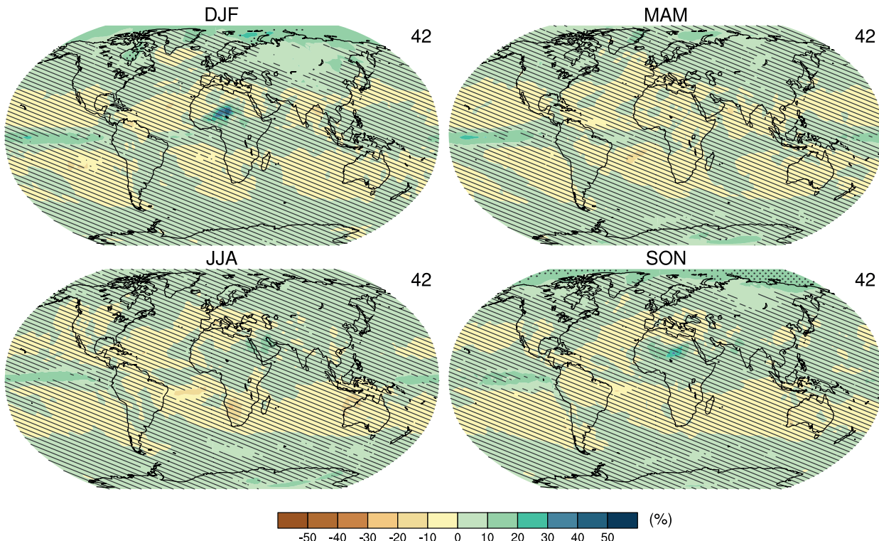
Figure 11.12 | CMIP5 multi-model ensemble mean of projected changes (%) in precipitation for 2016–2035 relative to 1986–2005 under RCP4.5 for the four seasons. The number of CMIP5 models used is indicated in the upper right corner. Hatching and stippling as in Figure 11.10.
