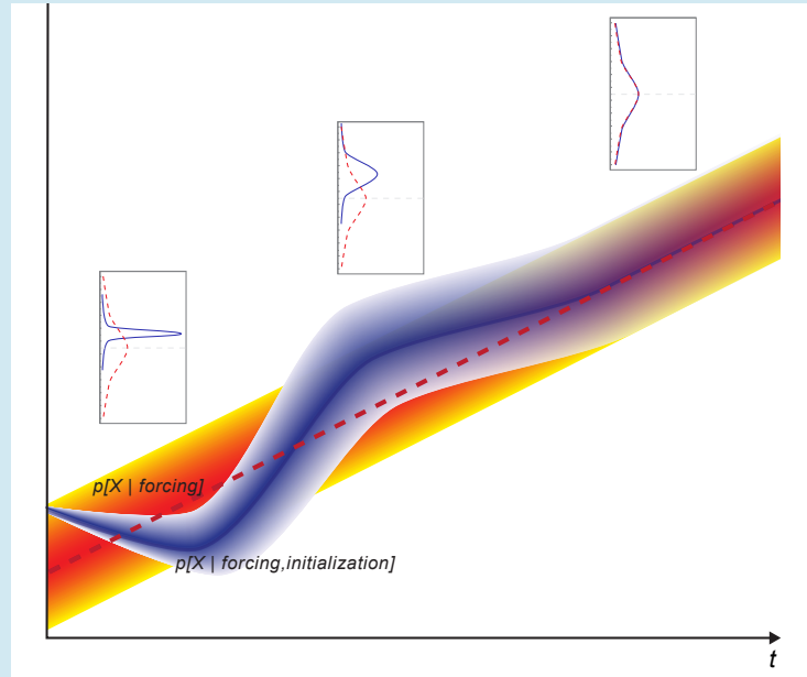
Box 11.1, Figure 3 | A schematic representation of prediction in terms of probability. The probability distribution corresponding to a forced simulation is in red, with the deeper shades indicating higher probability. The probabilistic forecast is in blue. The sharply peaked forecast distribution based on initial conditions broadens with time as the influence of the initial conditions fades until the probability distribution of the initialized prediction approaches that of an uninitialized projection. (Based on Branstator and Teng, 2010.)
