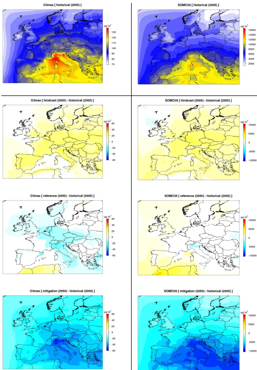
Fig. 3. Top row panels (from left to right): average fields of ozone as summertime average of the daily maxima ( \text{O}_3^{\text{max}} , \mu\text{g m}^{-3} ), and SOMO35 ( \mu\text{g m}^{-3} day) in the control (2005) simulation (averaged over 10 yr corresponding to the current climate). Following panel rows: difference between the simulations for the reanalysed ERA-hindcast and then for the reference and mitigation 2050 projections taken with respect to the GCM-historical climate simulation (2005). The differences are only displayed where significant given the interannual variability of 10 yr.
