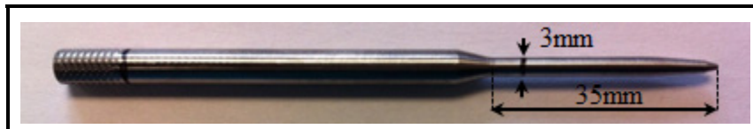
Figure 3.3 Custom-made indenter
