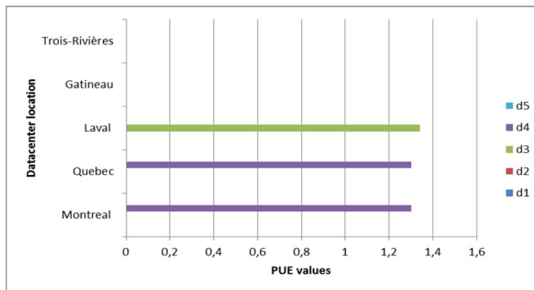
Figure-A I- 5 Power usage effectiveness (PUE) values
