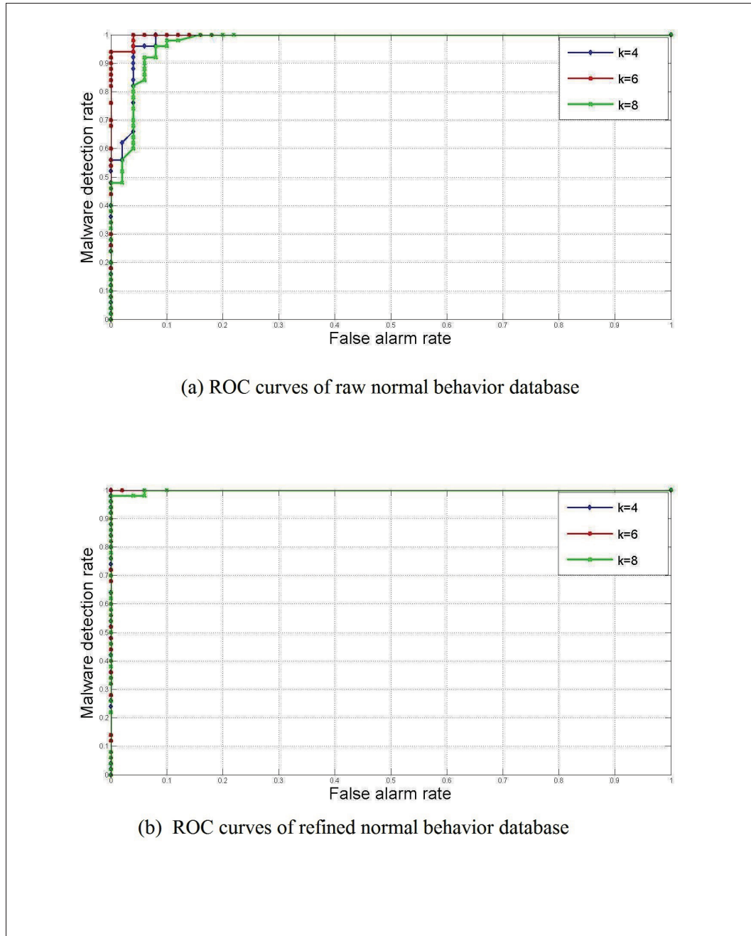
Figure 4.7 The ROC curves of the anomaly malware detection using the canonical benign behavior database approach
