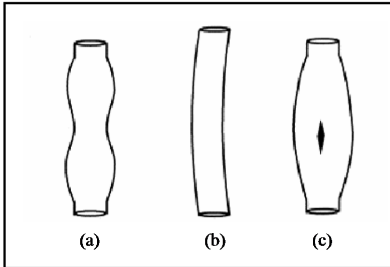
Figure 1.6: Failure modes in tube hydroforming: (a) wrinkling, (b) buckling, and (c) bursting (Koc and Altan, 2002).
