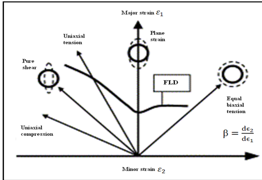
Figure 1.14: A typical Forming Limit Diagrams (FLD) along with different strain states (Holmberg, Enquist and Thilderkvist, 2004).
