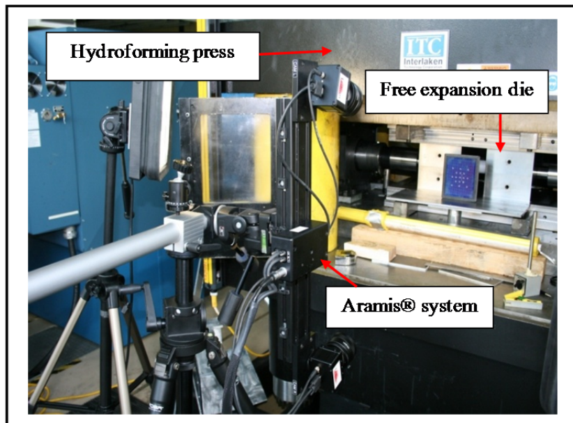
Figure 2.3: Experimental setup for the free expansion tests.
