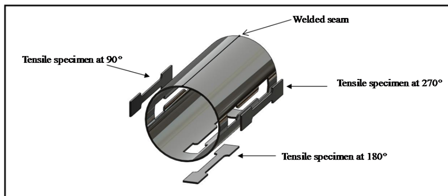
Figure 1.4: Schematic to show how tensile specimens are taken from a tube (Saboori et al., 2014a).
