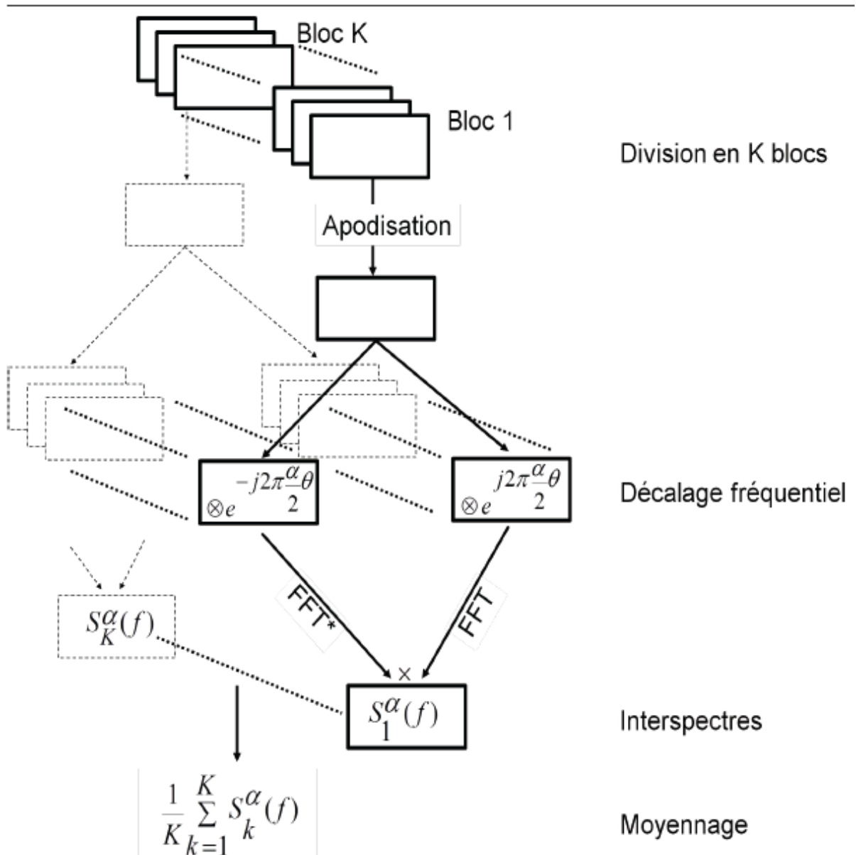
Figure 20 - Estimation de la corrélation spectrale.
