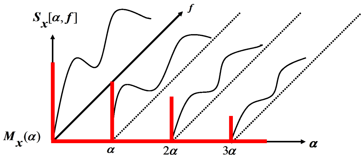
Figure 20 - Estimation de la corrélation spectrale.
