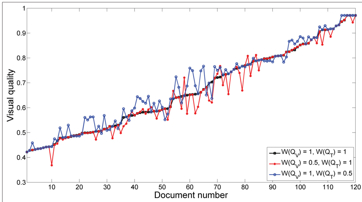
Figure D-7 JPEG optimal Q_V obtained by our framework (method 1) computed with a file size ratio of 1.15, N_B(D) = 50 kbps and N_L(D) = 488 ms. The slides are sorted according to the Q_V obtained using W_V(D) = 1, W_T(D) = 1 .
