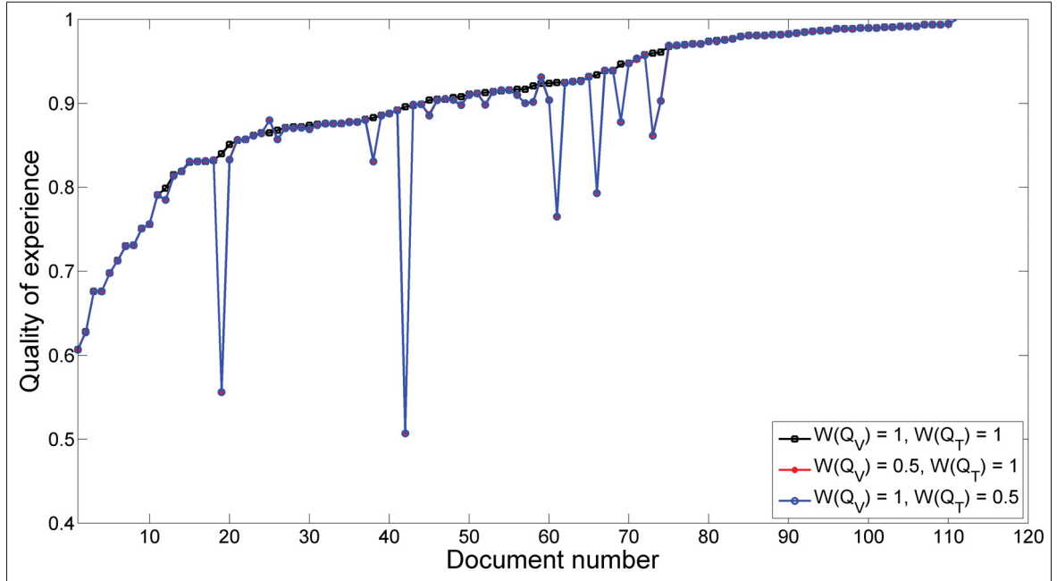
Figure D-12 XHTML optimal \mathcal{Q}_E obtained by our framework (method 1) computed with a file size ratio of 1, N_B(D) = 50 kbps and N_L(D) = 488 ms. The slides are sorted according to the \mathcal{Q}_E obtained using \mathcal{W}_V(D) = 1 , \mathcal{W}_T(D) = 1 .
