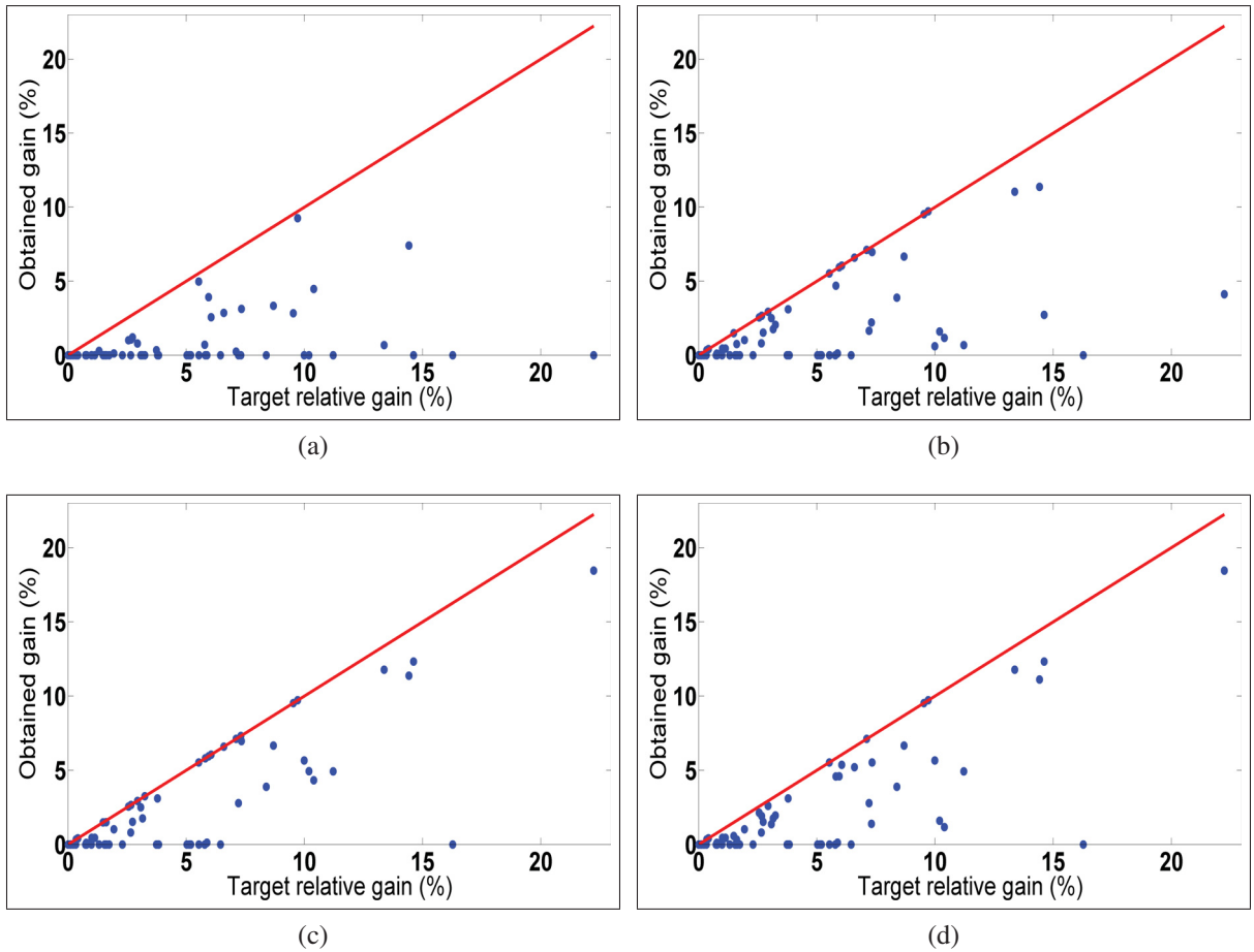
Figure 6.10 \mathcal{Q}_E relative gains for methods 2 to 5 with respect to method 1, when f_1^*(c_k, D) = \text{XHTML} .
