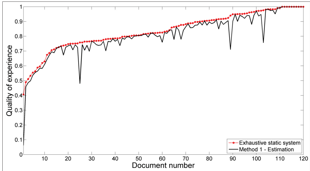
Figure D-2 XHTML optimal Q_E obtained by our framework (method 1) vs. that of the exhaustive static system computed with a file size ratio of 1, N_B(D) = 20 kbps and N_L(D) = 488 ms. The slides are sorted according to the Q_E of the exhaustive static system.
