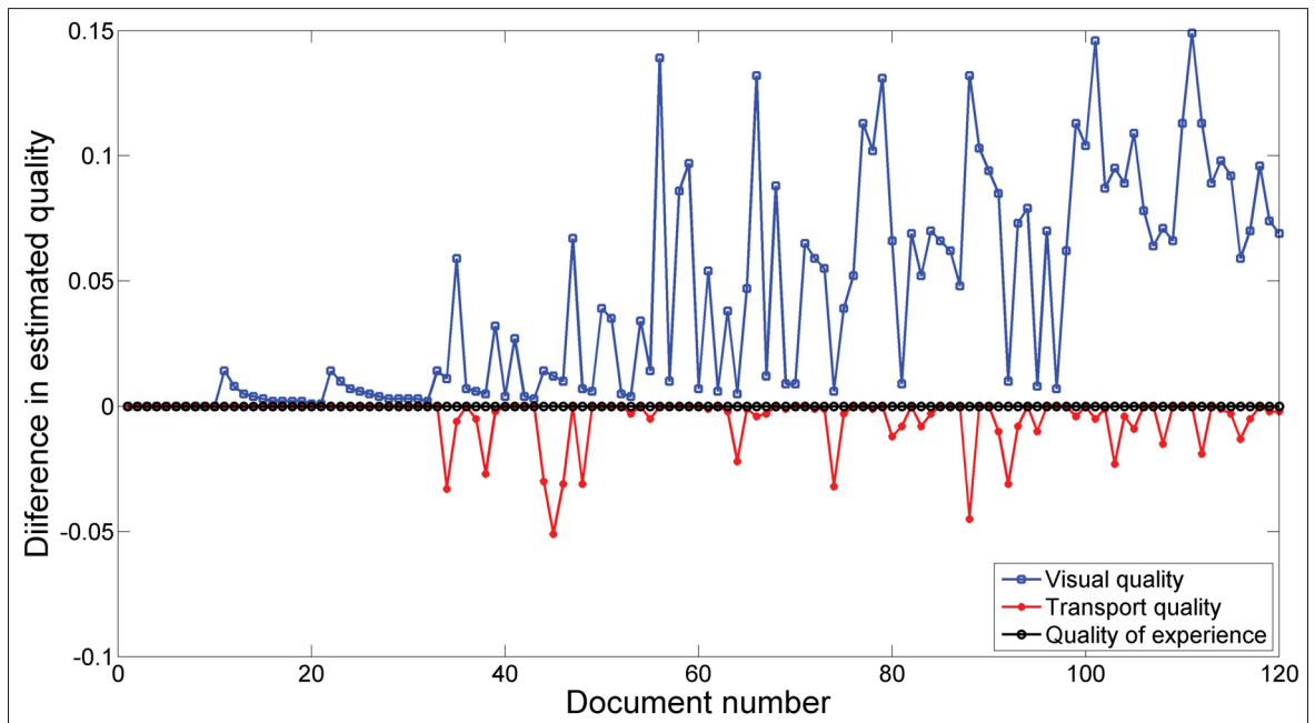
Figure D-13 Differences between the XHTML estimated \mathcal{Q}_V , \mathcal{Q}_T and \mathcal{Q}_E obtained with the two weight combinations ( \mathcal{W}_V(D) = 1 , \mathcal{W}_T(D) = 0.5 ) and ( \mathcal{W}_V(D) = 0.5 , \mathcal{W}_T(D) = 1 ), computed with a file size ratio of 1, N_B(D) = 50 kbps and N_L(D) = 488 ms.
