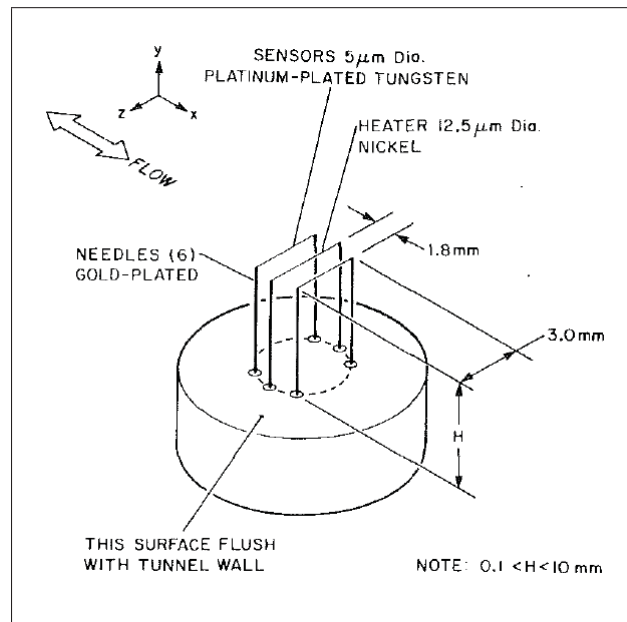
Figure 1.19 «Pushed Wall Probe» Tirée de Westphal et al. (1981)
