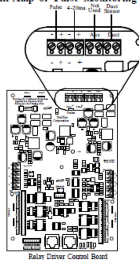
Relay Driver Control Board
