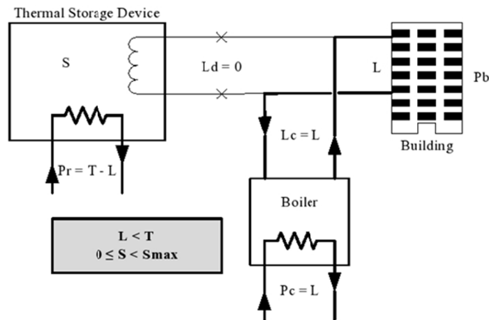
Figure 3. Thermal storage device recharges
