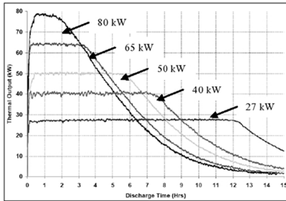
Figure 7. Supplied heating load, ThermElect ® 80 kW (Steffes Corporation, 2011)
