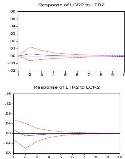
Figure 1B: Impulse response function
