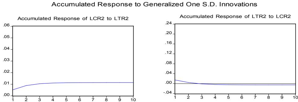
Figure 1A: Impulse response function { VAR(1) }
