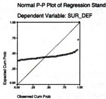
Figure 2: Normal Probability Plot of the Standardized Regression Residual.
