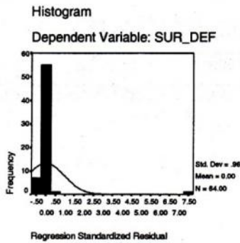
Figure 1: Visual identification of the shape of the Normal Distribution.
