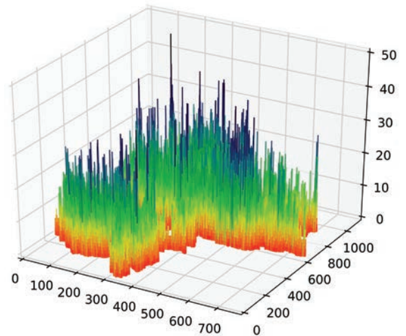
Figure 5. A “random” walk on a million digits of Catalan’s constant.
