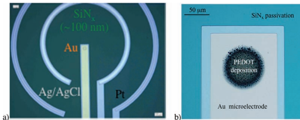
Fig. 1. Optical microscope images of (a) the integrated (Au-Pt-Ag/AgCl) electrochemical microcell (ElecCell) device and (b) the electrodeposited PEDOT film on the gold working electrode (solvent: acetonitrile)
