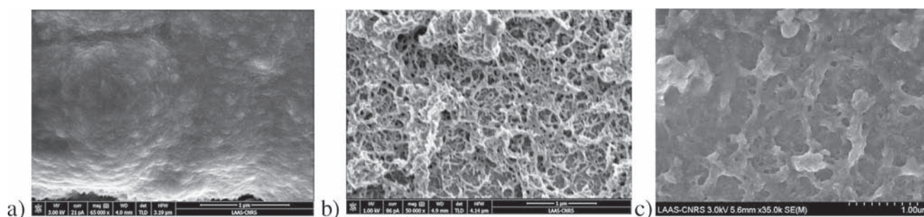
Fig. 3. Scanning electron microscopy (SEM) pictures of PEDOT films deposited on (a) on gold surface using water as solvent, (b) on gold surface using acetonitrile as solvent and (c) on platinum surface while using acetonitrile as solvent
