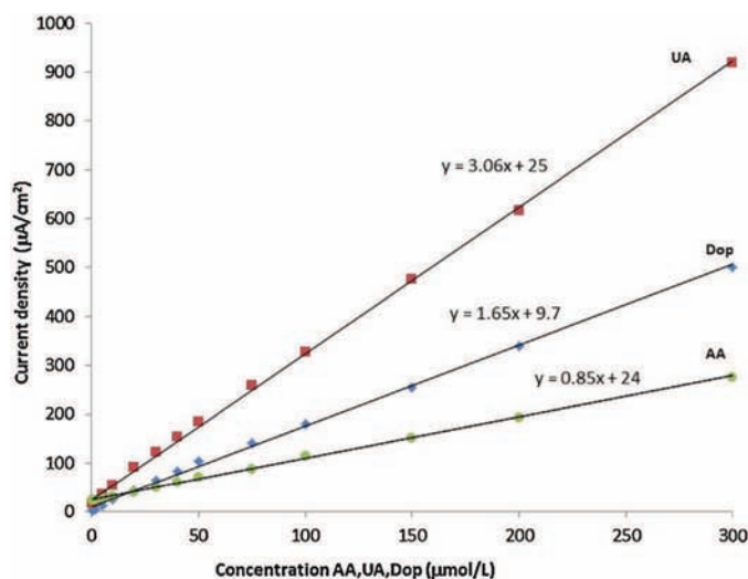
Fig. 8. Calibration curves for the three analytes: ascorbic acid, dopamine and uric acid.
