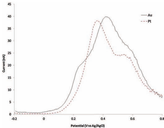
Fig. 5. Differential pulse voltammograms (DPV) of (Au-Pt-Ag/AgCl) (plain line) and (Pt-Pt-Ag/AgCl) (dashed line) ElecCell in 0.1 M PBS pH 7.0 solution containing an equimolar AA/Dop/UA mixture (1 mmol/L).
