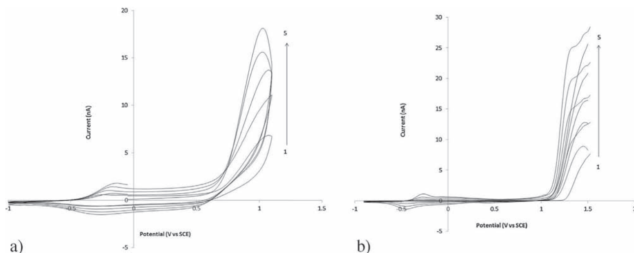
Fig. 2. Cyclic voltammograms of electropolymerization at gold working microelectrode in deaerated 0.1 mol/L TBAPC and 2.5 mmol/L EDOT (a) water-based (potential scan rate: 25 mV/s) and (b) acetonitrile-based solutions (potential scan rate: 250 mV/s).
