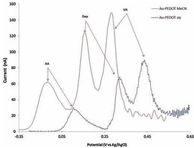
Fig. 4. Differential pulse voltammograms (DPV) of (Au/PEDOT-Pt-Ag/AgCl) ElecCell in 0.1 M PBS pH 7.0 solution containing an equimolar AA/Dop/UA (1 mmol/L): PEDOT electrodeposited in acetonitrile solution (plain line) or in aqueous solution (dashed line).
