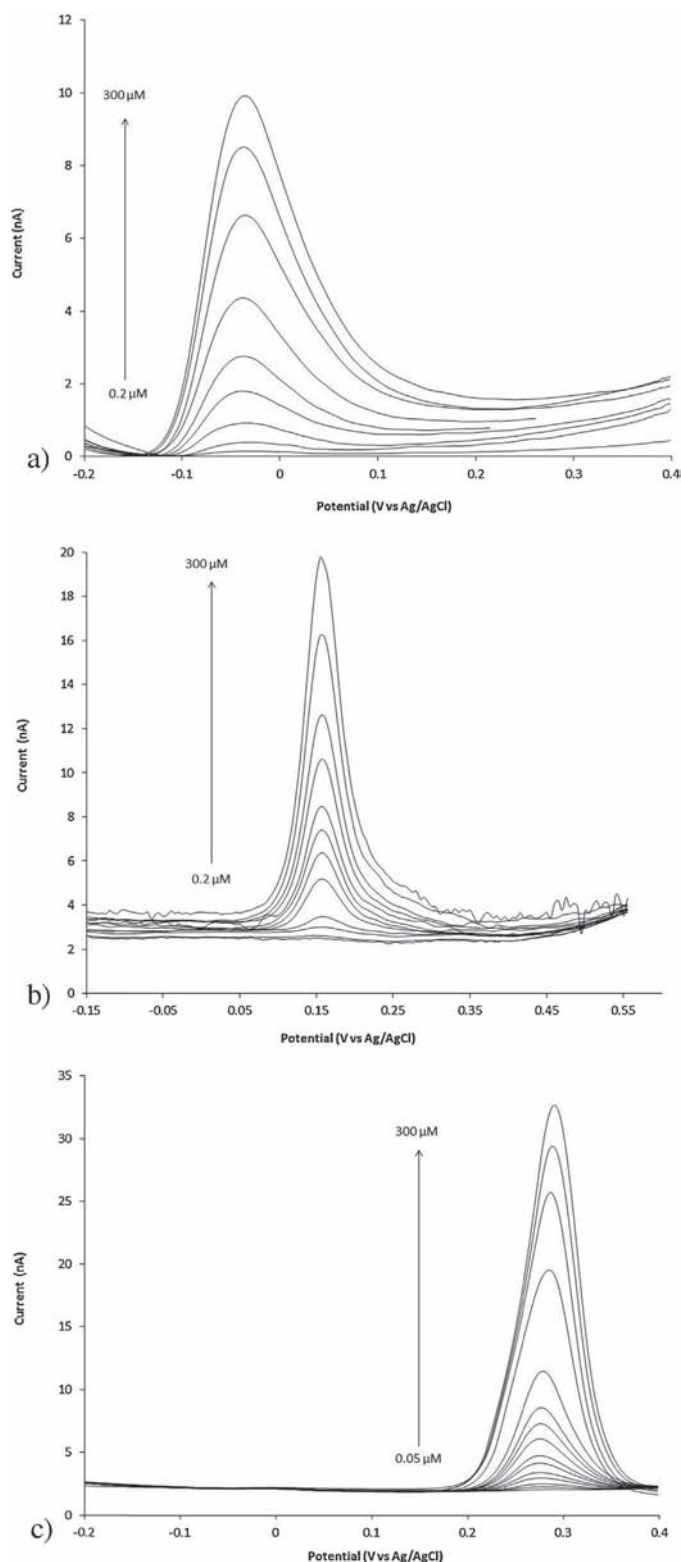
Fig. 7. Differential pulse voltammograms of (Au/PEDOT-Pt-Ag/AgCl) elecCell in 0.1 M PBS (pH 7.0) containing different concentrations of (a) ascorbic acid, (b) dopamine and (c) uric acid.
