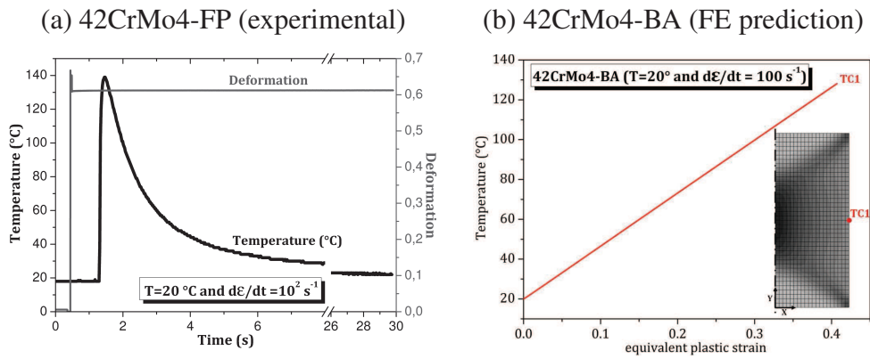
Figure 11: Increase of the temperature during deformation due to self-heating for a compression test at T = 20^\circ\text{C} and \dot{\varepsilon} = 10^2 \text{ s}^{-1} . Comparison between (a) The experimental measurement the 42CrMo4-FP steel and (b) The FE prediction for the 42CrMo4-BA steel.
