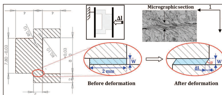
Figure 6: Theoretical shear zone.
