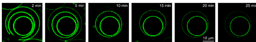
Figure 8. 18:1-NBD-PE incorporated into encapsulated POPC/27-OH-cholesterol (chol) GUV membranes quenched by dithionite. The images (from left to right) highlight a sequence of pictures collected in time after addition of the quencher to the space outside the multivesicular liposome. Measurements were performed at 25 °C.
