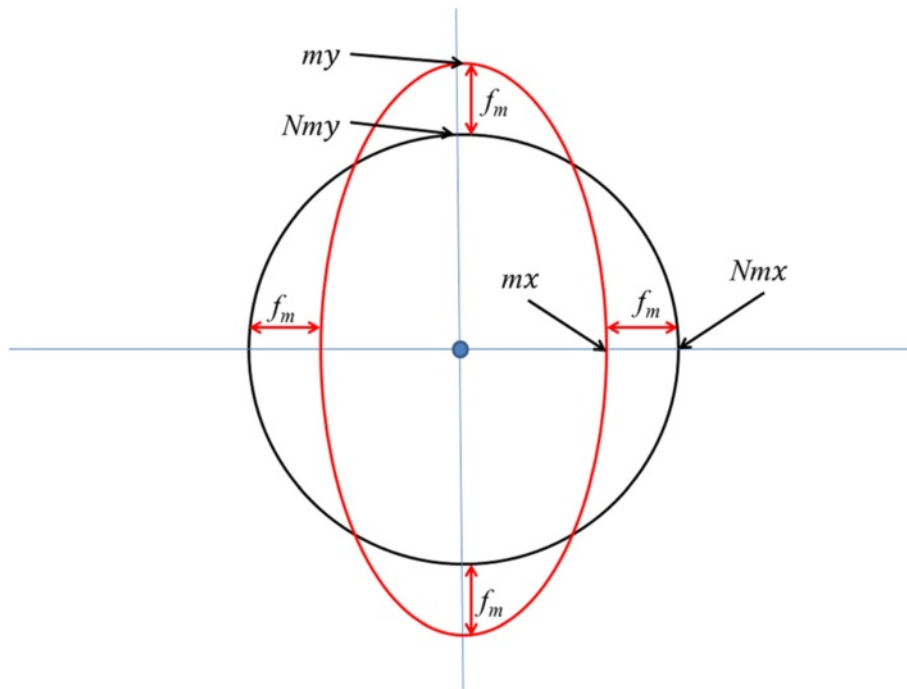
Fig. 4 Visualisation of magnetometer data where distortions in the magnetic field due to soft iron sources near to the sensors may change the expected outputs on the various axes (two of three shown for simplicity). This can be corrected by appropriate normalising procedure (see text)
