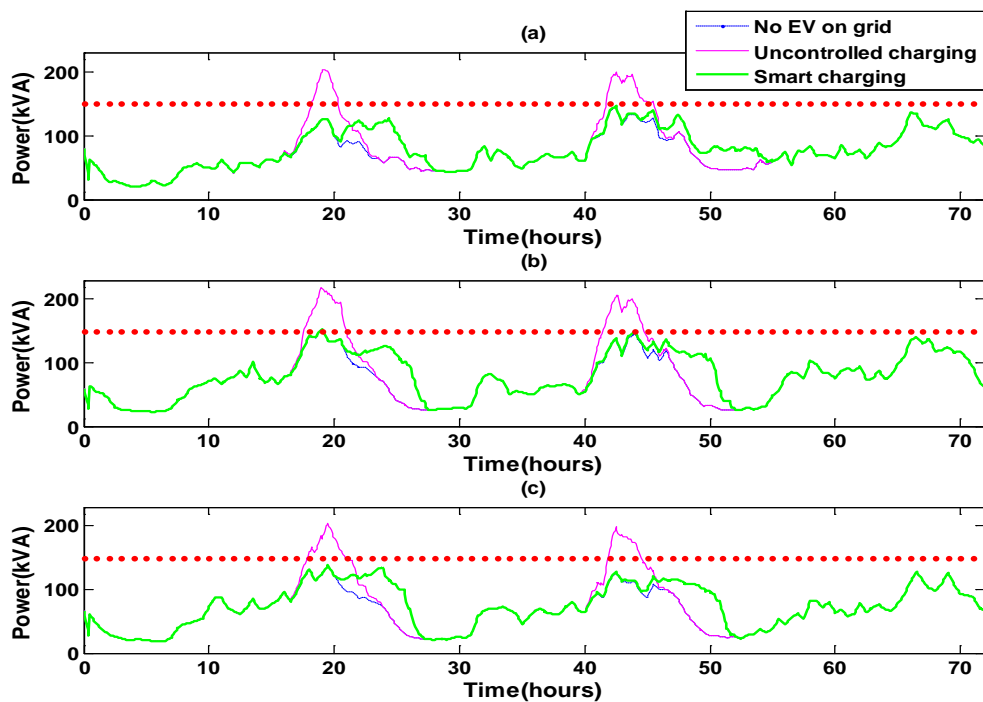
Figure 13 Distribution transformer power flows with and without EV charging superimposed (AIMD-GIVP smart charging, winter scenario): (a) residential area A; (b) residential area B; (c) residential area C.
