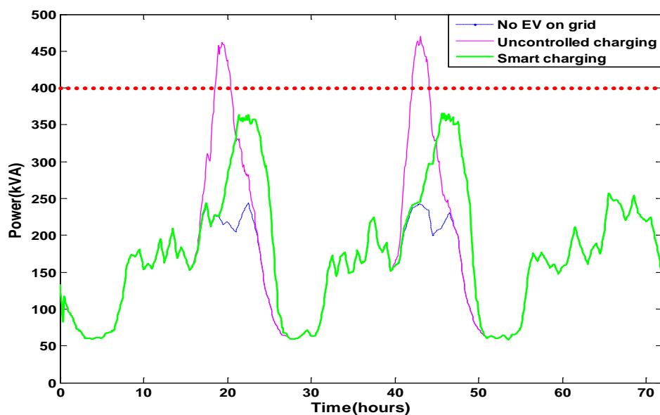
Figure 9 Main Substation power flow with and without EV charging superimposed (AIMD-GIVP smart charging, summer scenario)
