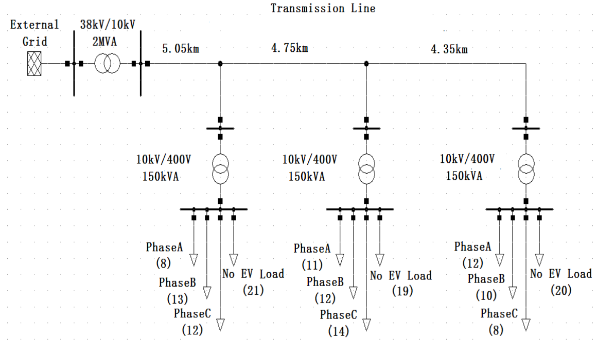
Figure 5 Schematic diagram of the distribution network
