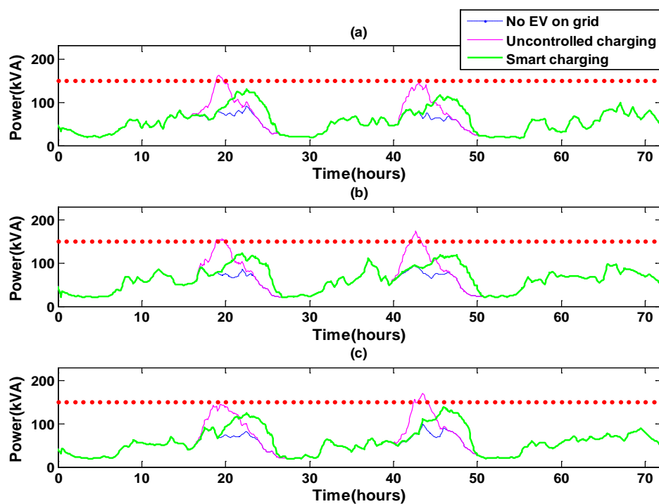
Figure 9 Main Substation power flow with and without EV charging superimposed (AIMD-GIVP smart charging, summer scenario)
