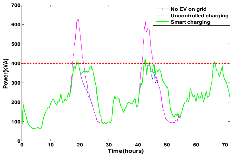
Figure 12 Substation power flow with and without EV charging superimposed (AIMD-GIVP smart charging, winter scenario)
