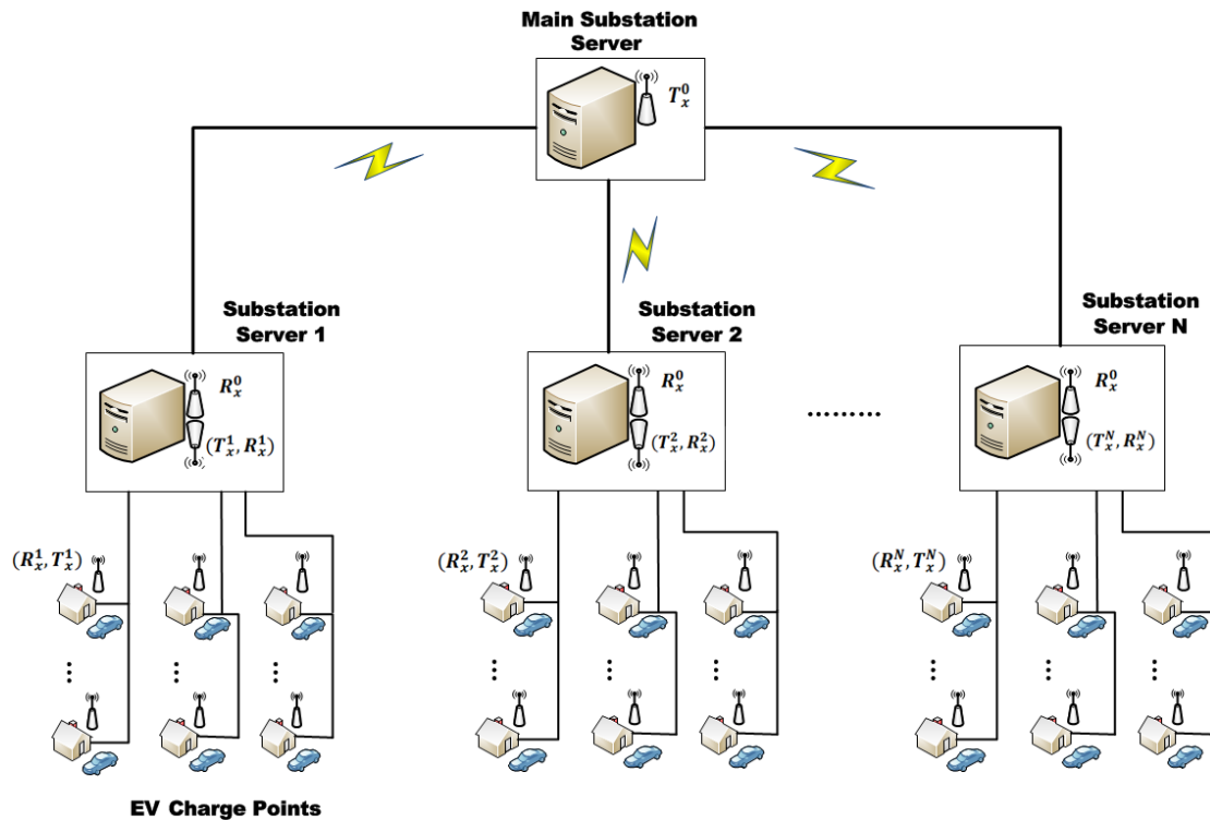
Figure 3 Communication topology for the Enhanced AIMD implementation
