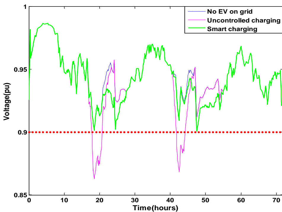
Figure 11 Minimum voltage level on residential area buses with and without EV charging superimposed (AIMD-GIVP smart charging, winter scenario)
