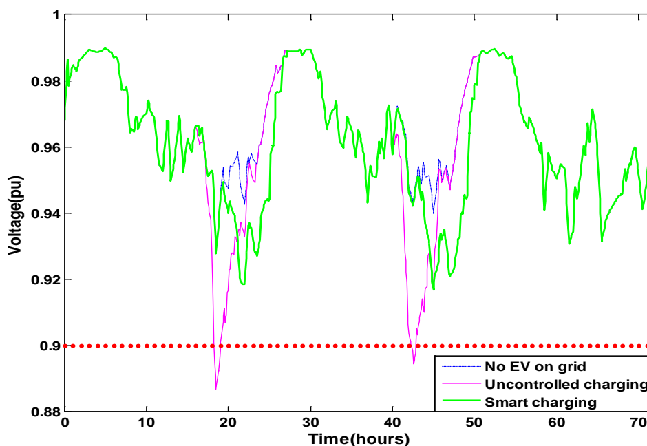
Figure 8 Minimum voltage level on residential area buses with and without EV charging superimposed (AIMD-GIVP smart charging, summer scenario)
