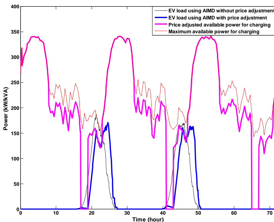
Figure 15 Comparison between EV loads obtained using Enhanced AIMD smart charging with and without price adjusted available power (summer scenario).
