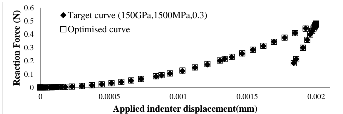
Figure 7.3 Comparison between experimental data and optimised data after iterations (Target values, E = 150GPa, \sigma_y = 1500MPa and 'n' =0.3)
