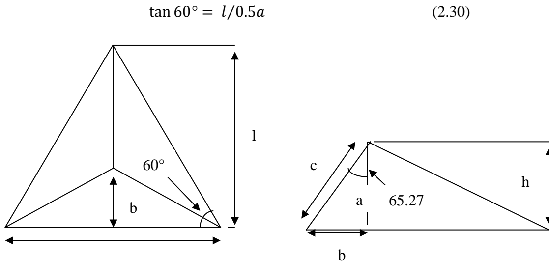
Figure 2.5 Berkovich indenter
