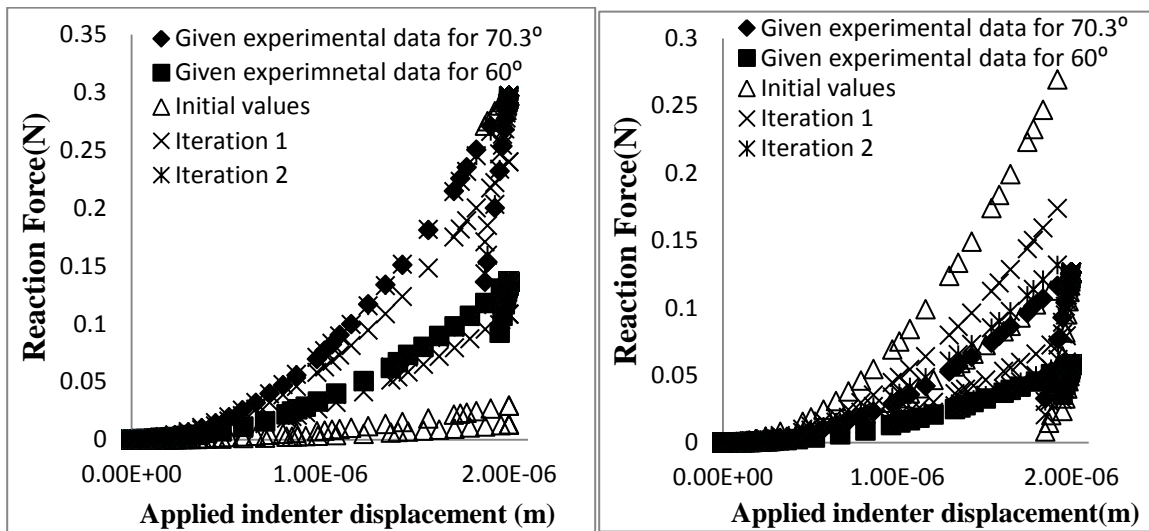
Figure 6.19 Optimisation results and target loading-unloading curve using dual indenters (a) E = 100\text{GPa} , \sigma_y = 900\text{MPa} and 'n' =0.3 (b) E = 50\text{GPa} , \sigma_y = 300\text{MPa} and 'n' =0.4
