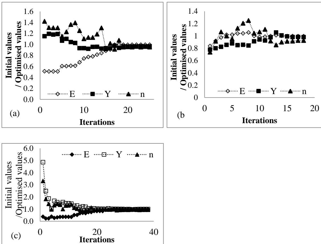
Figure 9.5 Optimised parameter values versus iterations for test 3(a) case 1, (b) case 2 and (c) case 3 using Optimisation Method 1
