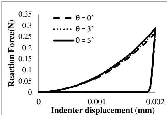
Figure 4.12 Influence of tilted indenter on loading-unloading curves of indentation. (a) Conical indenter (b) Berkovich indenter (c) Vickers indenter (d) Flat-ended 60^\circ cone indenter with force control
