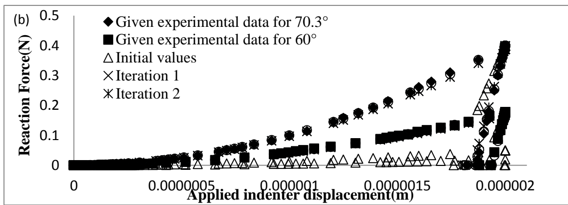
Figure 6.12 Optimisation results and target loading-unloading curve using dual indenters (a) E = 50\text{GPa} , \sigma_y = 300\text{MPa} and n = 0.1 (b) E = 210\text{GPa} , \sigma_y = 900\text{MPa} and n = 0.3
