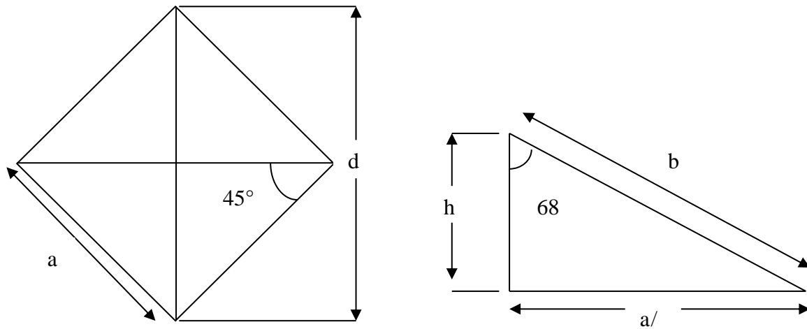
Figure 2.6 Vickers indenter
