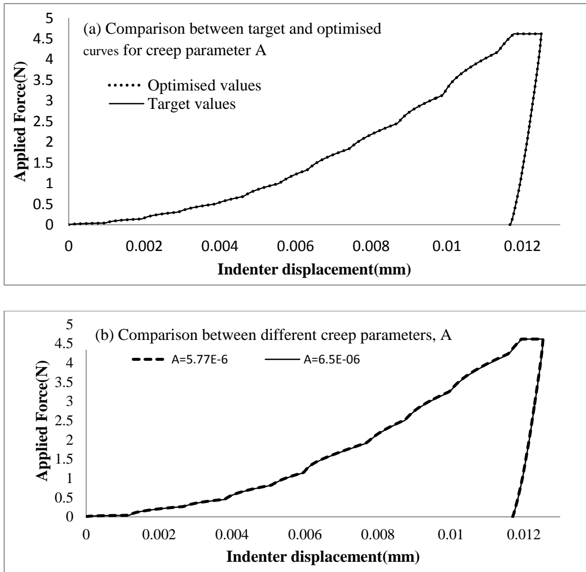
Figure 8.9 (a) Comparison between target and optimised curves for creep parameter, A, for a spherical indenter (b) Indentation curves obtained from two different creep parameters, A, for a spherical indenter.
