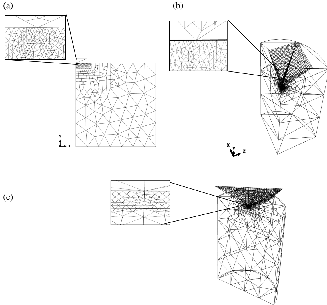
Figure 4.4. Typical FE meshes used in the indentation analysis (a) axisymmetric conical indenter (b) 3D Vickers indenter (c) 3D Berkovich indenter
