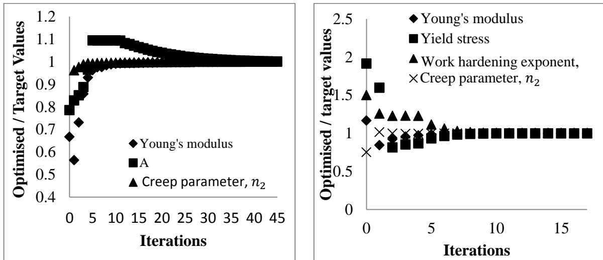
Figure 8.6 Optimised parameter values versus iterations for a spherical indenter (a) Test 3 and (b) Test 4
