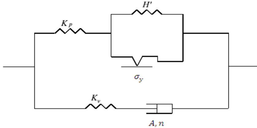
Figure 8.1 One-dimensional idealization of the two-layer viscoplasticity model [89]
