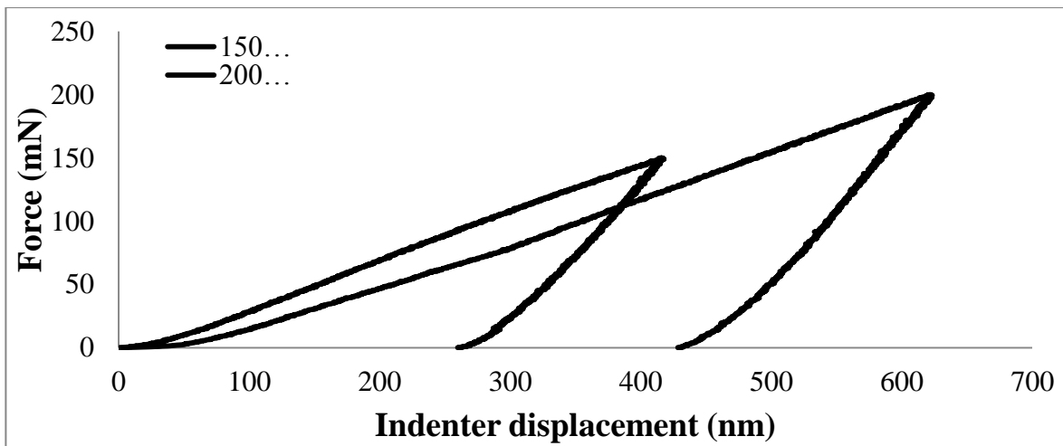
Figure 9.1 Experimental loading-unloading curves at different load levels using (a) Berkovich and (b) Spherical indenters
