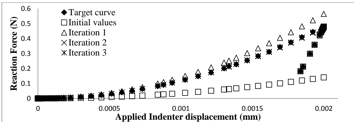
Figure 7.2 Optimisation results and target loading-unloading curve of material properties (Target values, E = 150GPa, \sigma_y = 1500MPa and 'n' =0.3)
