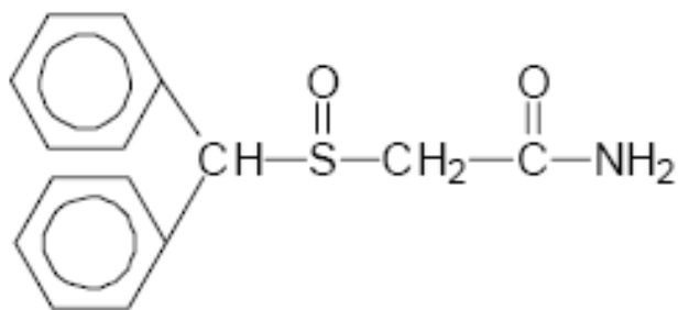
Figure 1.6 Chemical structure of modafinil.
