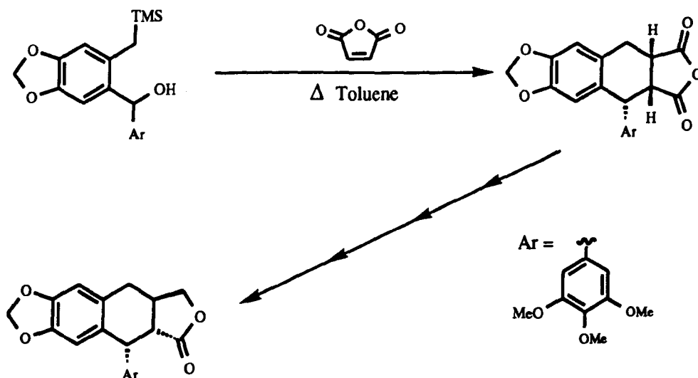
(Scheme 25)
