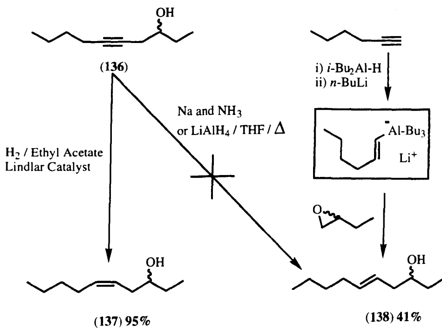
(Scheme 13)
