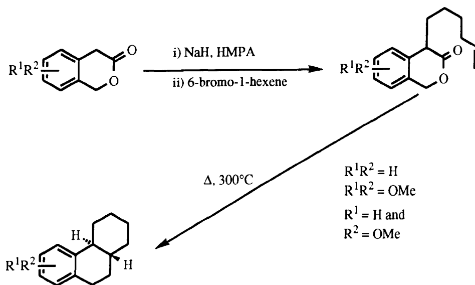
(Scheme 7)
