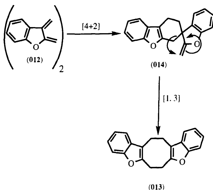
( Scheme 14 )
