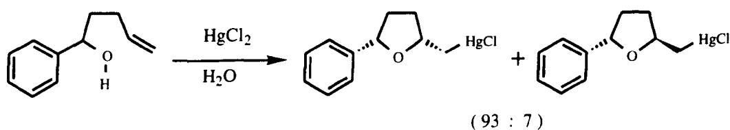
(Scheme 25)
