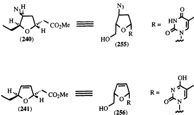
( Scheme 58 )
