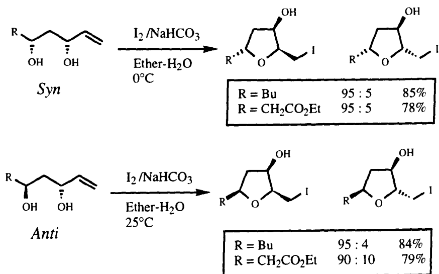
(Scheme 6)
