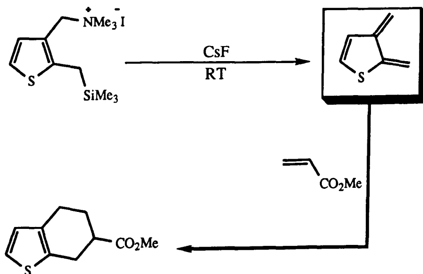
( Scheme 50 )
