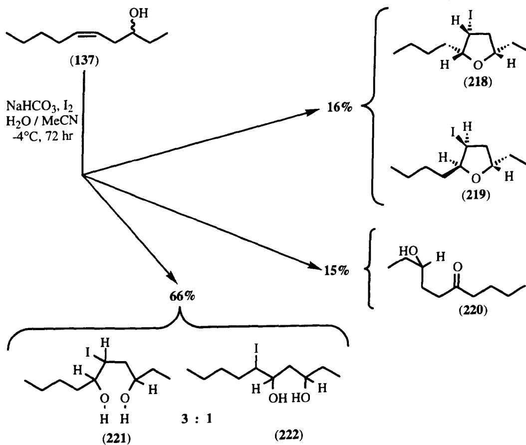
( Scheme 43 )
