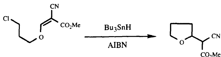
( Scheme 45 )
