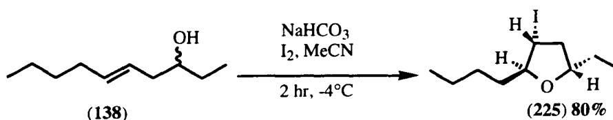
( Scheme 46 )
