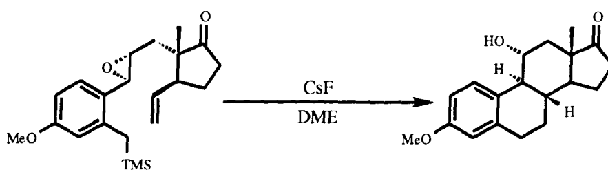
( Scheme 23 )
