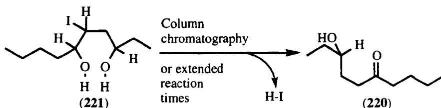
( Scheme 44 )
