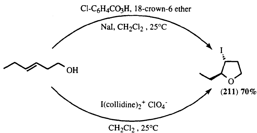
( Scheme 41 )
