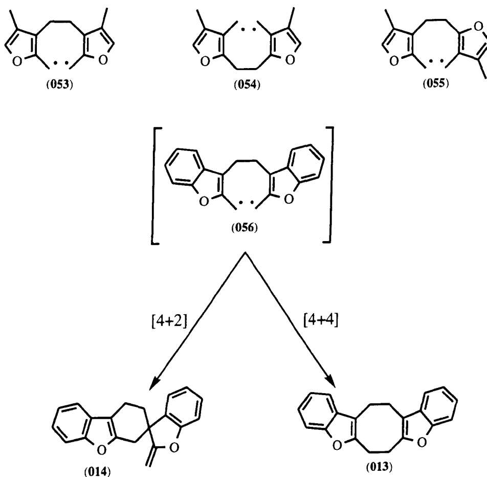
( Scheme 21 )
