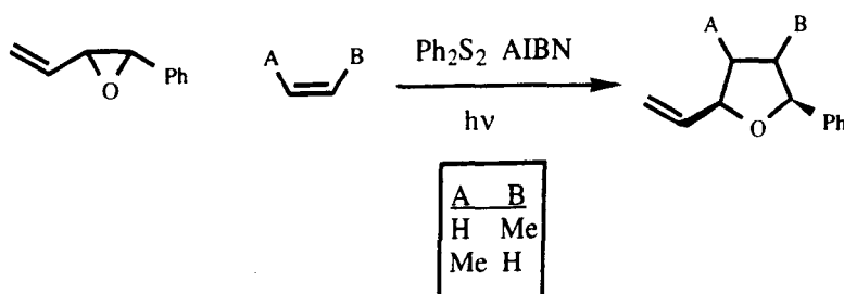
( Scheme 47 )
