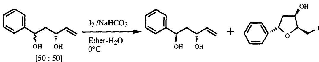
(Scheme 7)
