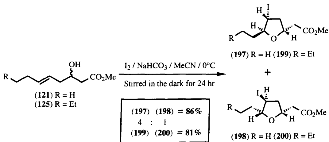
( Scheme 32 )
