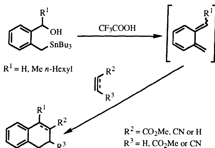
(Scheme 14)
