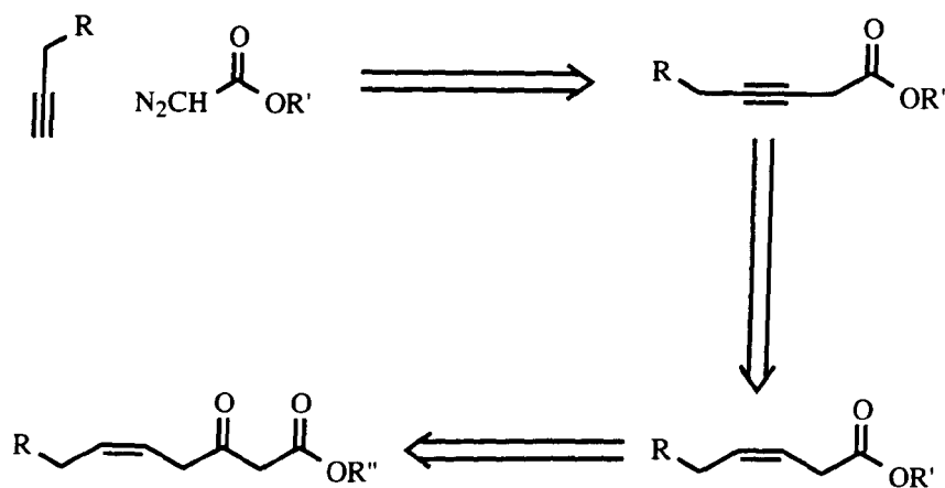
(Scheme 6)
