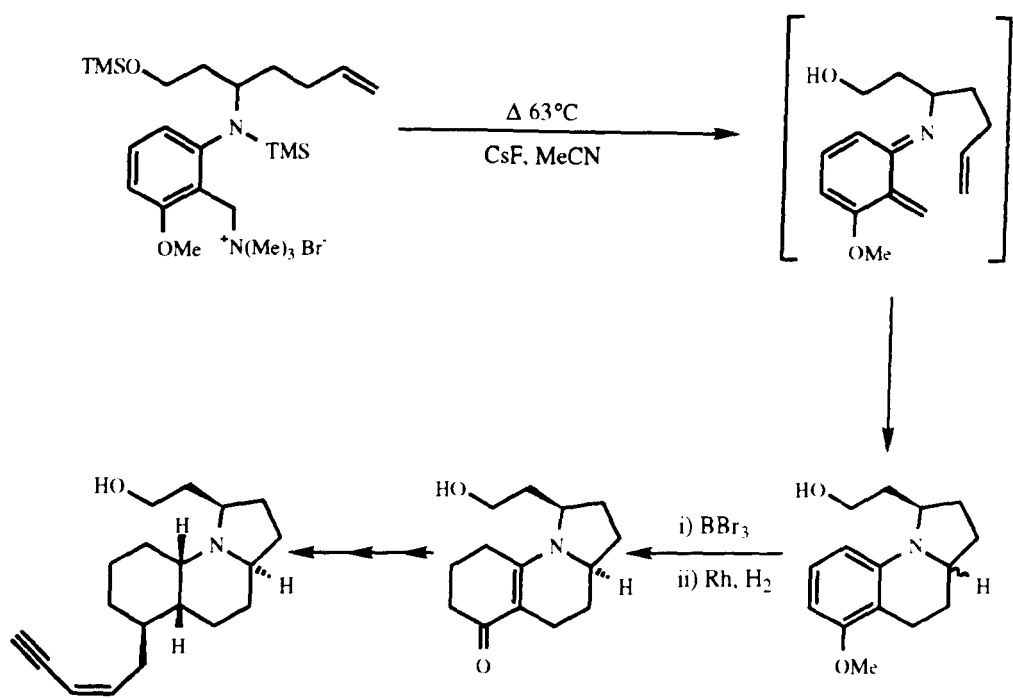
( Scheme 27 )
