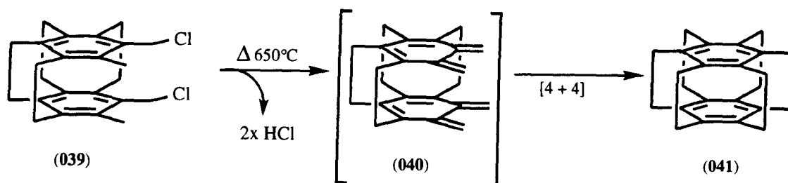
( Scheme 15 )
