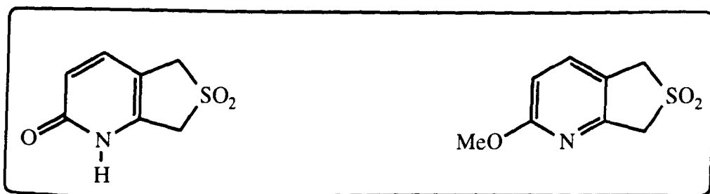
( Scheme 41 )
