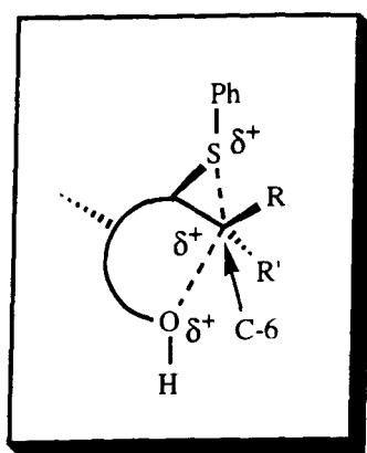
( Scheme 20 )
