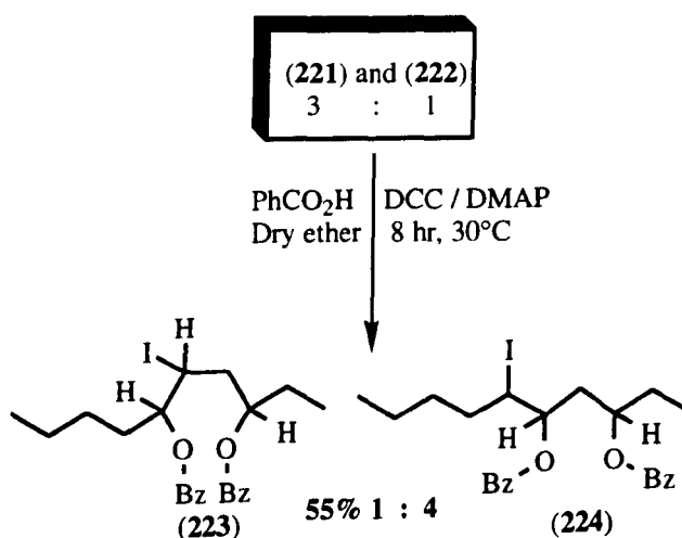
( Scheme 45 )
