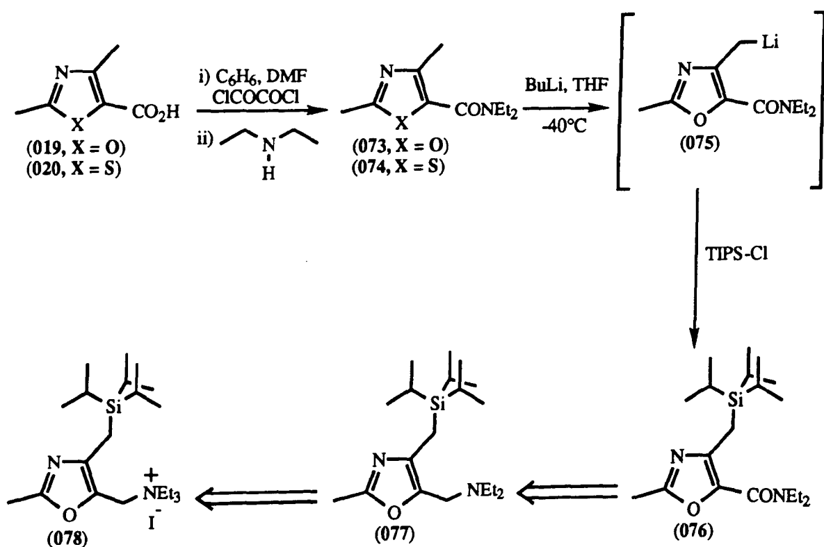
( Scheme 30 )
