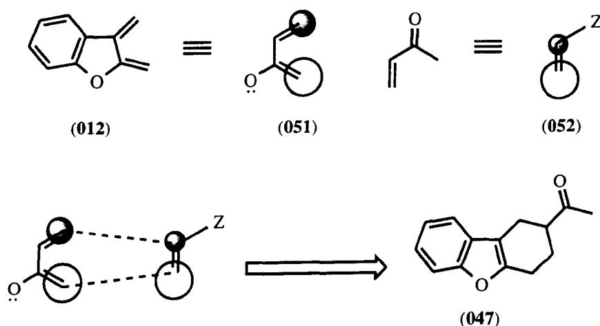
( Scheme 20 )
