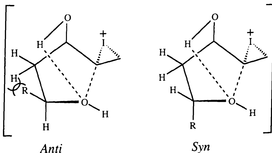
(Scheme 8)
