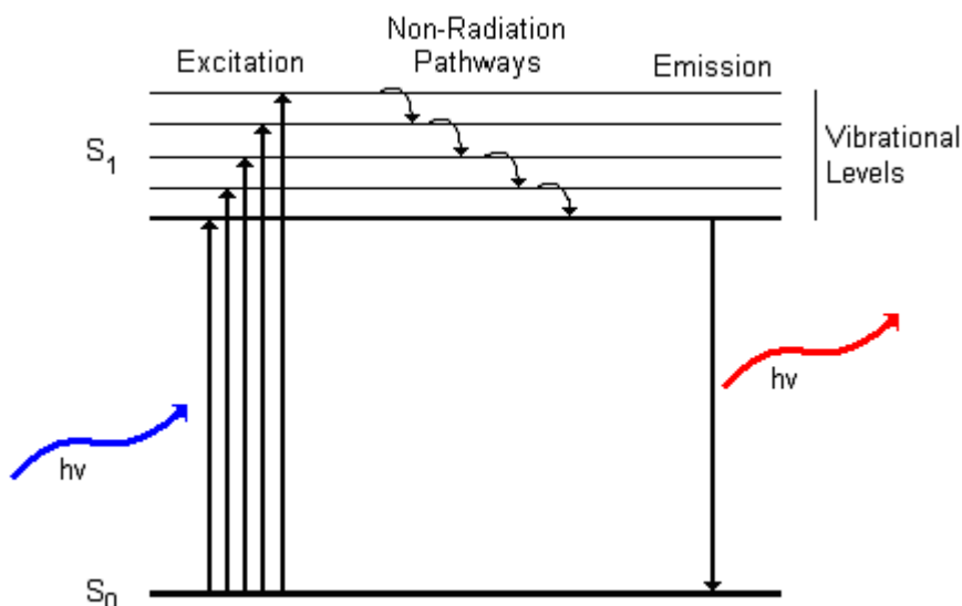
Figure 1.11 Excitation and emission of fluorescent molecules.
