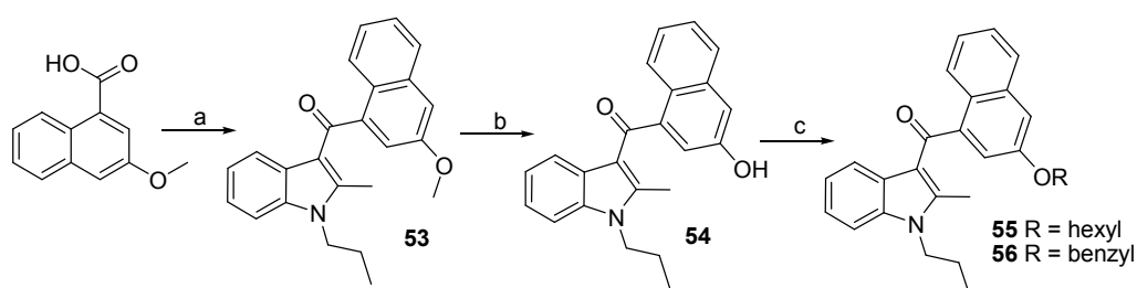
Scheme 2.7 Synthesis of 2-methyl- N -propyl-3-(3-alkoxy-1-naphthoyl)-indoles (a) (i) SOCl 2 , reflux; (ii) 32 , Et 2 AlCl, DCM (90 %); (b) BBr 3 , DCM (71 %). (c) NaH, DMF, 1-BrR, (16-32 %).
