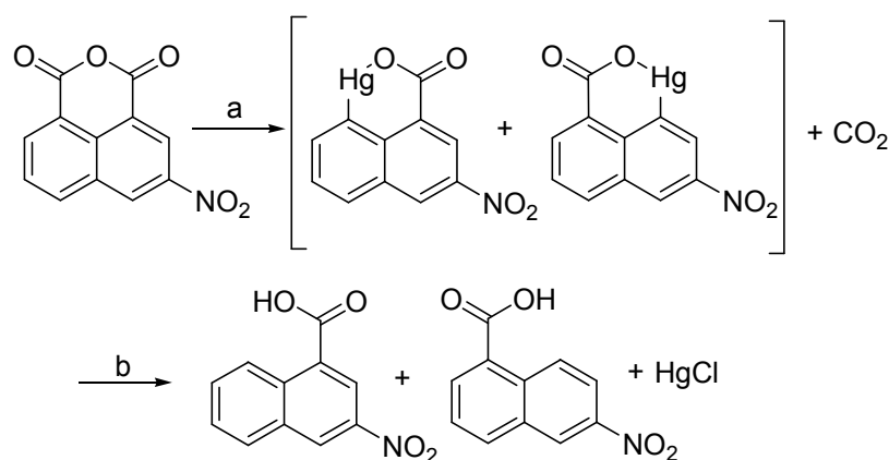
Scheme 2.6 Selective decarboxylation of 3-nitro-1,8-naphthoic anhydride 47 (a) (i) NaOH (aq) ; (ii) HgO, 3:1 AcOH:H 2 O, reflux (b) HCl, reflux.
