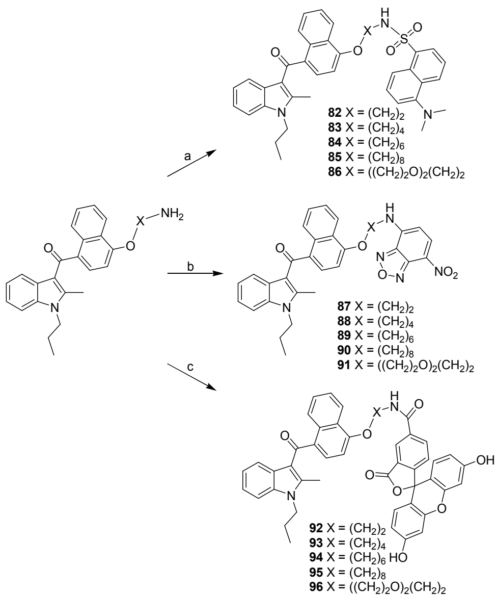
Scheme 3.5 Preparation of fluorescent JWH-015 analogues (a) dansyl chloride, TEA, DCM, (29-46 %); (b) 4-fluoro-7-nitrobenzofurazan TEA, DCM, (15-29 %); 5-carboxyfluorescein- N -succinimdy ester, TEA, DCM, (80-96 %).
