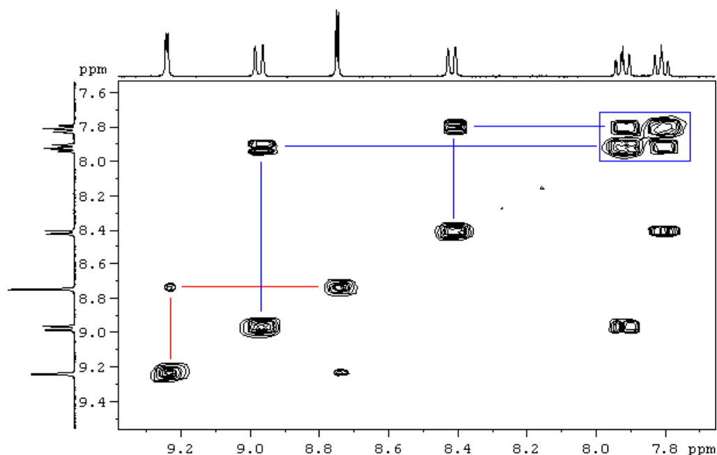
Figure 2.8 COSY NMR of 3-nitro-1-naphthoic acid 48 , with H^1 NMR on left and top axis. Red lines show coupling between 2-H and 4-H, and blue lines show coupling between 5-H, 6-H, 7-H and 8-H.
