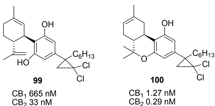
Figure 4.4 CB 2 receptor selective modifications at C 1 position. Receptor binding affinities (K i ) quoted.
