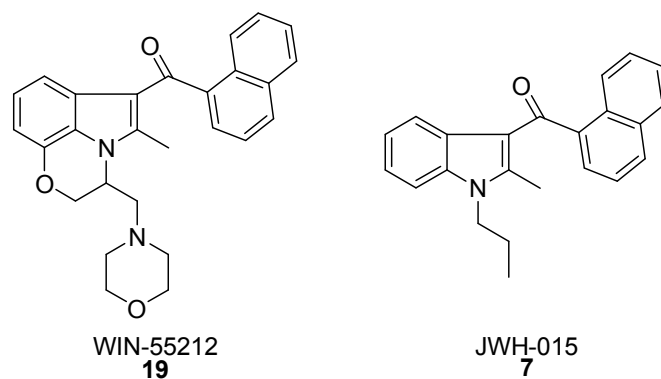
Figure 1.9 Examples of alkyndole cannabinoids.
