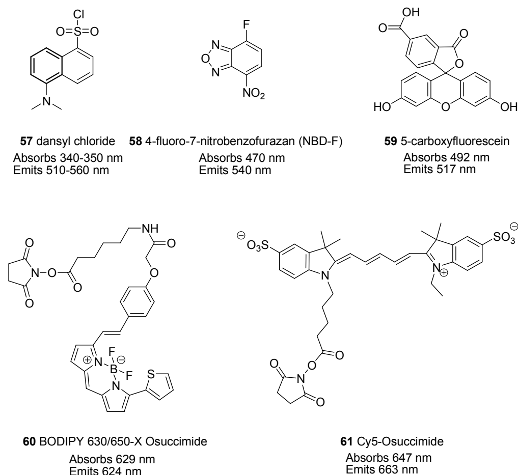
Figure 3.1 Structure and spectral data for amine reactive fluorophores. \lambda_{\max} absorbances and emission are quoted. Dansyl chloride and NBD-F data taken from Lakowicz 139 , and, as dansyl chloride alone is non-fluorescent, a range of values of its conjugates are given. 5-carboxyfluorescein data is taken from product specifications of Sigma-Aldrich 140 , and Bodipy 630/650-X Osuccimide and Cy5-Osuccimide data taken by work from Buschmann et al 141 .
