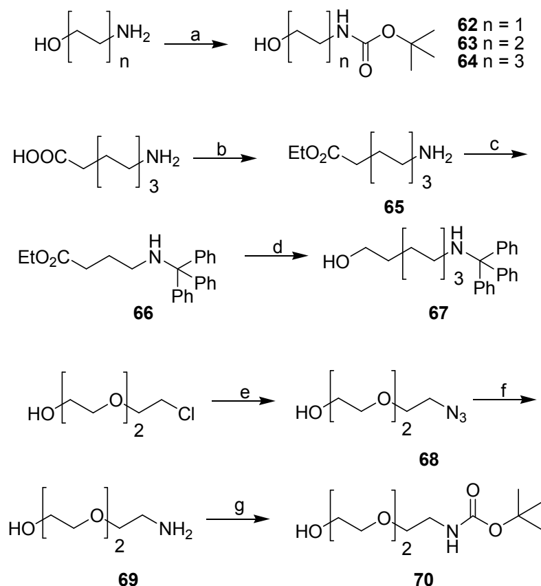
Scheme 3.2 Synthesis of N - t -butoxycarbonyl or N -trityl protected linkers (a) t -butylphenyl carbonate, TEA, EtOH n=1 (76 %), n=2 (65 %), n=3 (96 %); (b) PTSA, EtOH, reflux, (96 %); (c) trityl chloride, TEA, \text{CHCl}_3 , (89 %); (d) \text{LiAlH}_4 , THF, (65 %); (e) \text{NaN}_3 , DMF, (99 %); (f) \text{SnCl}_2 , EtOH, (54 %), or \text{Ph}_3\text{P} , \text{H}_2\text{O} , ether, reflux (31 %); (g) di- t -butyl dicarbonate, \text{KOH}_{(\text{aq})} , (68 %).
