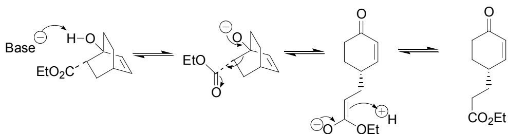
Figure 4.11 Base catalysed reverse Claisen rearrangement to form cyclohexanone 112 .
