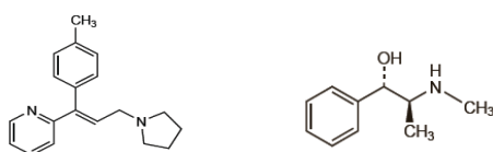
Triprolidine (TRI) Pseudoephedrine (PSE) Fig 1: Chemical structures of triprolidine and pseudoephedrine
