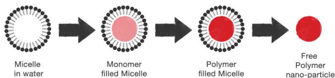
Figure 9. Schematic illustrating the steps by which the soft template method produces CP nanoparticles.
