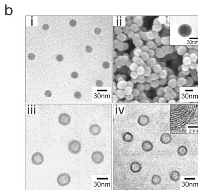
Figure 10. a) Schematic illustrating the fabrication of polypyrrole nano-particles, hollow nano-capsules and their carbon derivatives. b) SEM and TEM micrographs of (i) polypyrrole nano-particles, (ii) linear polypyrrole/cross-linked polypyrrole core/shell nanoparticles, (iii) polypyrrole nano-capsules, and (iv) carbon nanocapsules. Reproduced from Ref. 64 with permission from The Royal Society of Chemistry.
