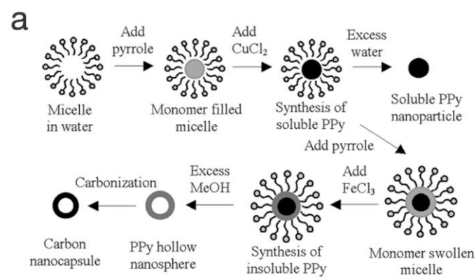
Figure 9. Schematic illustrating the steps by which the soft template method produces CP nanoparticles.
