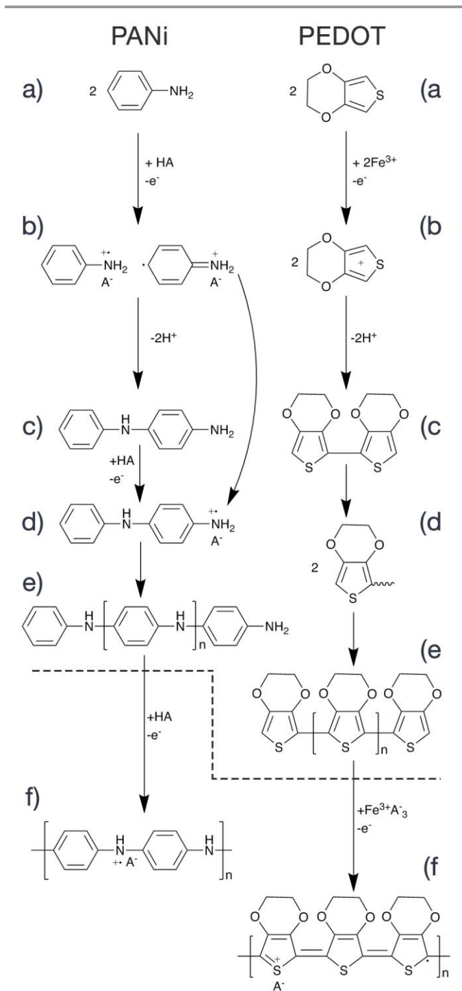
Figure 6. Schematic of the proposed polymerisation mechanism of PANi and PEDOT
