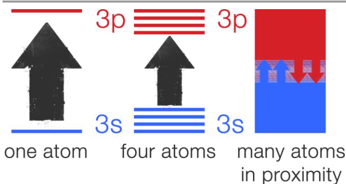
Figure 2. Schematic showing the formation of bands in conducting materials (e.g. sodium) according to Quantum theory. When many atoms are in close proximity to each other their atomic orbitals overlap and form a mixed orbital 'band'. The blue lines and box represent electron filled orbital(s) and the red lines and box represent unfilled orbital(s). The arrows represent the movement of electrons between orbitals.
