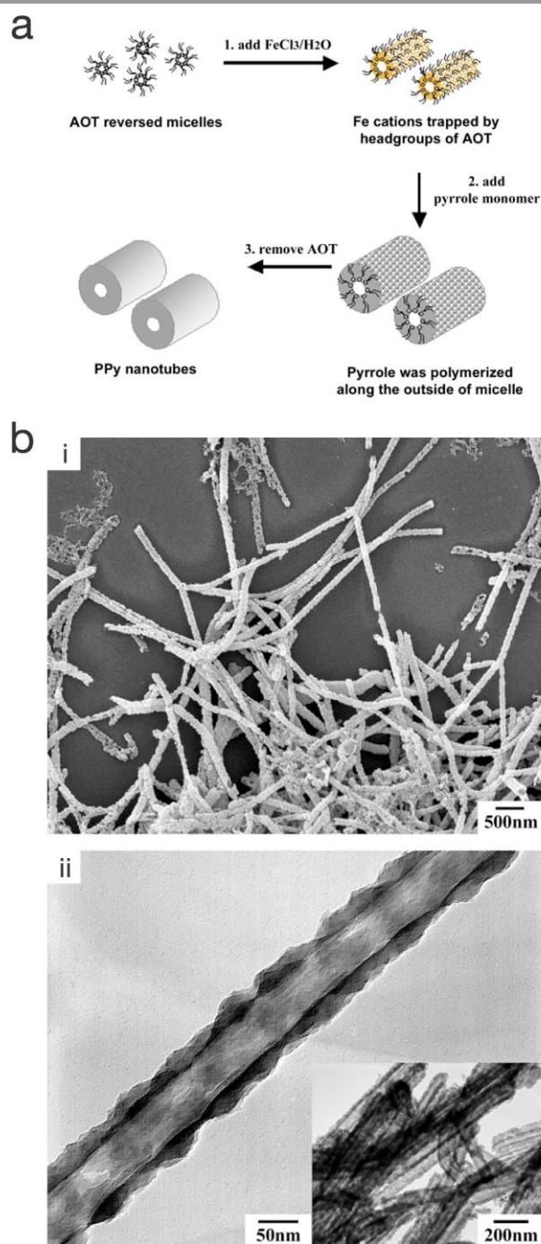
Figure 11. a) Schematic illustrating the fabrication of polypyrrole hollow nanotubes via reversed micelle polymerisation. b) (i) SEM micrograph of polypyrrole nanotubes, and (ii) TEM micrograph of a polypyrrole nanotube. Reproduced from Ref. 67 with permission from The Royal Society of Chemistry.
