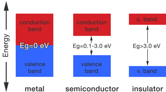
Figure 4. Energy band diagram demonstrating different band gap energies
