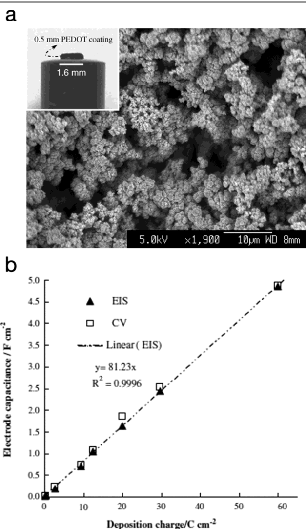
Figure 18. a) SEM micrograph of PEDOT electropolymerised via potentiostatic polymerisation (deposition charge: 30 \text{ C cm}^{-2} ). Inset: photograph of a PEDOT film ( 60 \text{ C cm}^{-2} ) on a Pt disc electrode. b) Plot of the electrode specific capacitance as a function of polymerisation charge. Values measured by electrochemical Impedance Spectroscopy (EIS) and Cyclic Voltammetry (CV) are both presented. Reprinted from Ref. 89 with permission from Elsevier.
