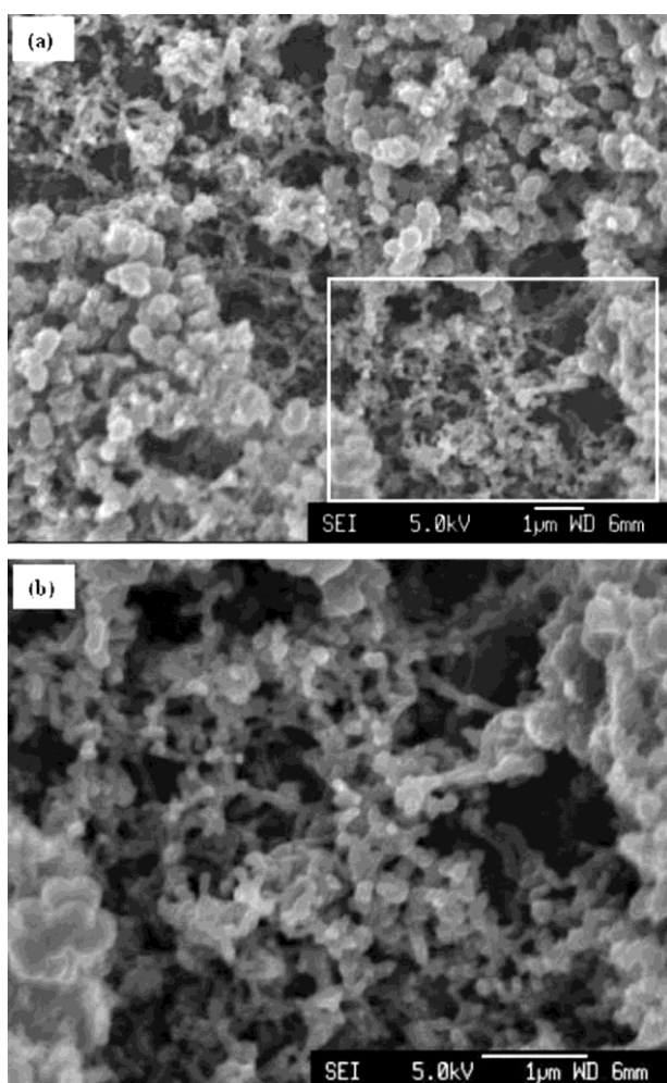
Figure 17. SEM micrographs of (a) the surface of a MWNT-PANi polymerised via galvanostatic polymerisation at 1 mA for 5 min, and (b) higher magnification of the rectangle in (a), showing the nanoporous network of MWNTs-PANi composite. Reproduced from Ref. 42 with permission from The Royal Society of Chemistry.
