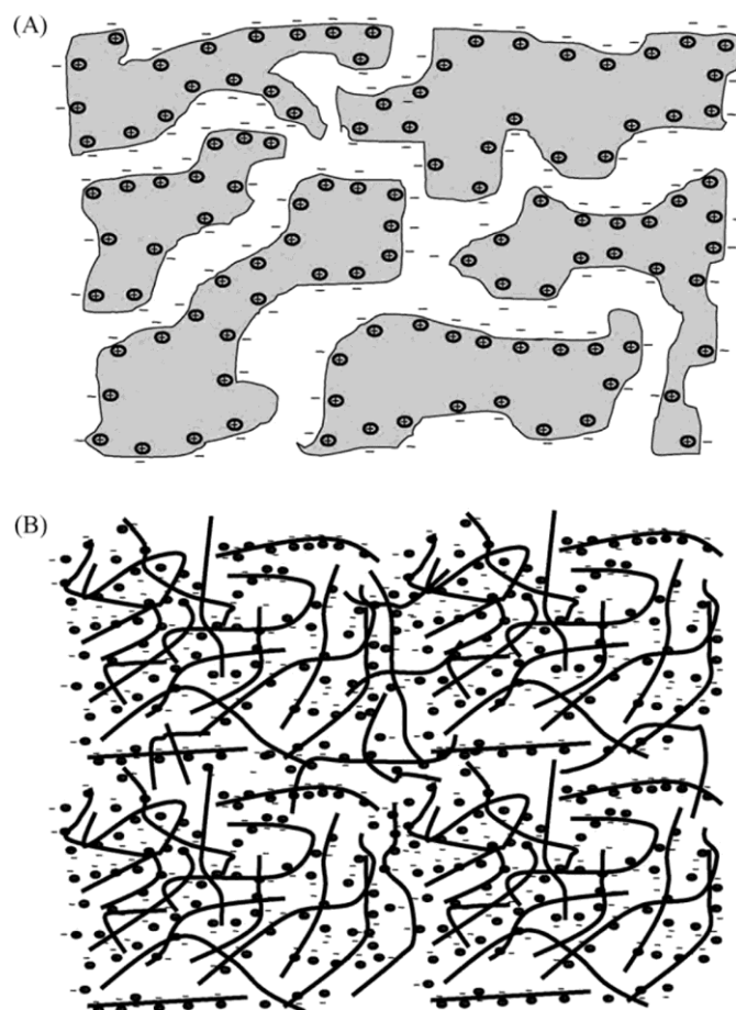
Figure 16. Illustration of the mechanism of charging of (a) EDLCs (carbon), and (b) pseudo-capacitor (CPs). Reprinted from Ref. 78 with permission from Elsevier.
