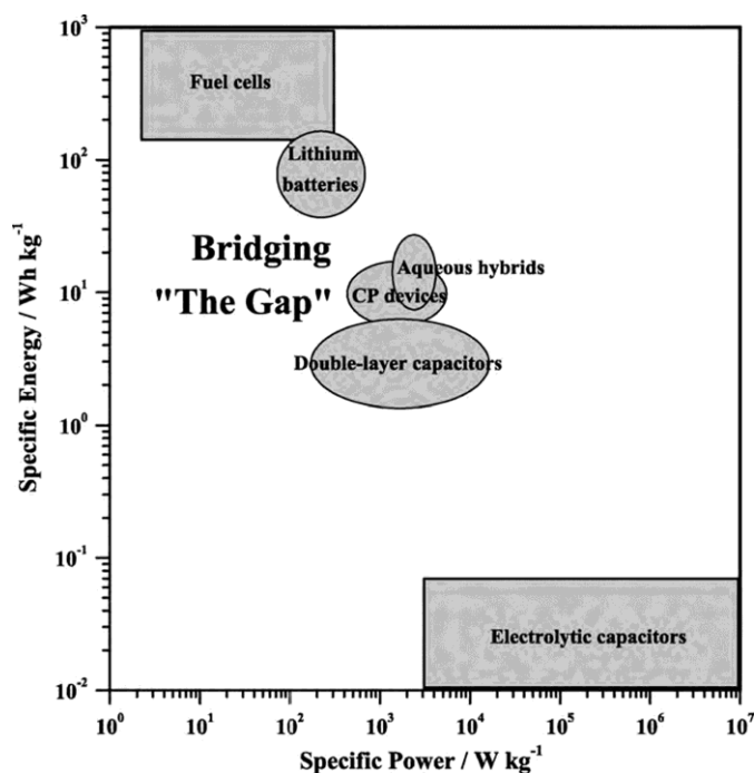
Figure 15. Ragone plot illustrates different types of energy-storage devices as a function of specific power and energy. Reprinted from Ref. 78 with permission from Elsevier.
