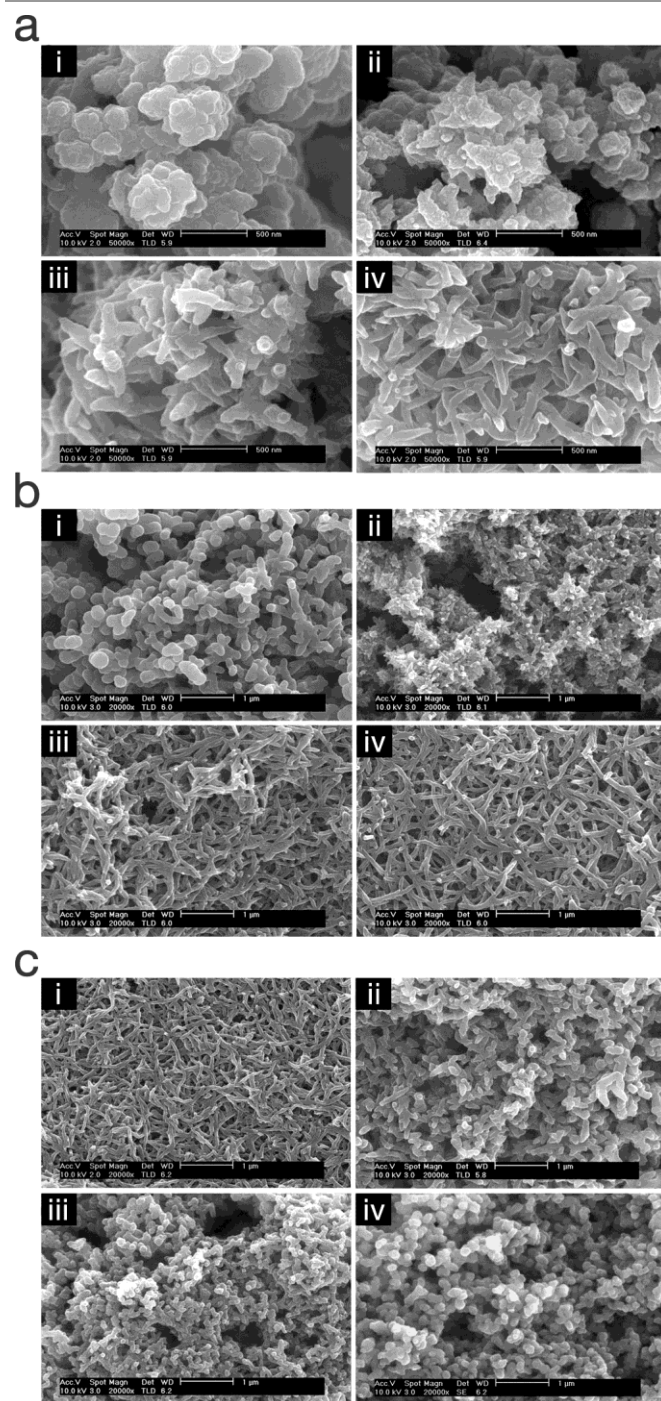
Figure 13. SEM micrographs of polypyrrole nanostructures electropolymerised under different conditions; a) polymerisation time (i) 1 min, (ii) 2 min, (iii) 3 min, and (iv) 4 min., b) pyrrole concentration (i) 0.025 M, (ii) 0.05 M, (iii) 0.10 M, and (iv) 0.20 M., and c) dopant concentration (i) 0.20 M, (ii) 0.40 M, (iii) 0.60 M, and (iv) 0.80 M. Reproduced from Ref. 71 with permission from The Royal Society of Chemistry.
