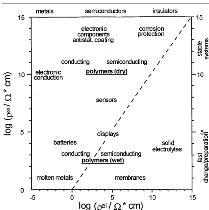
Figure 14. Double logarithmic plot outlines the applications of CPs as a function of ionic (y-axis) and electronic resistances (x-axis). Reprinted from Ref. 74 with permission from Elsevier.
