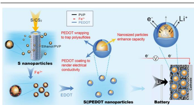
Figure 20. Illustration of the preparation of sulphur/PEDOT core/shell nanoparticles and their application as cathode materials. On the left, the synthesis of sulphur nanoparticles via a membrane-assisted precipitation method is shown. In the middle, the encapsulation of the sulphur nanoparticles with a PEDOT shell via oxidation polymerisation. On the right, sulphur/PEDOT nano-particles as the cathode material that allows electron transport and Li ions to diffuse while limiting the polysulfide dissolution is shown. Reprinted by permission from Macmillan Publishers Ltd: Scientific Reports 97 , copyright (2013)
