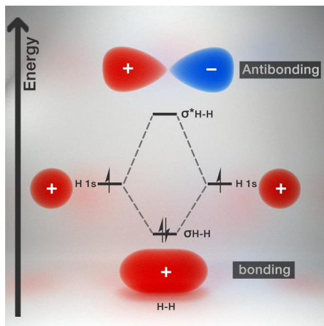
Figure 3. Diagram of the molecular orbitals of the hydrogen molecule
