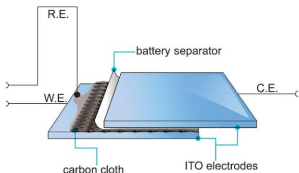
Figure 22. Illustration of the electropolymerisation method used to polymerise PEDOT onto carbon cloths. The carbon cloth is wetted with EDOT in C4mpyrTFSI IL or 1 M LiTFSI in acetonitrile and covered with a battery separator from one side and then sandwiched between two ITO-glass electrodes. Reprinted by permission from Wiley: ChemPlusChem 4 , copyright (2015)
