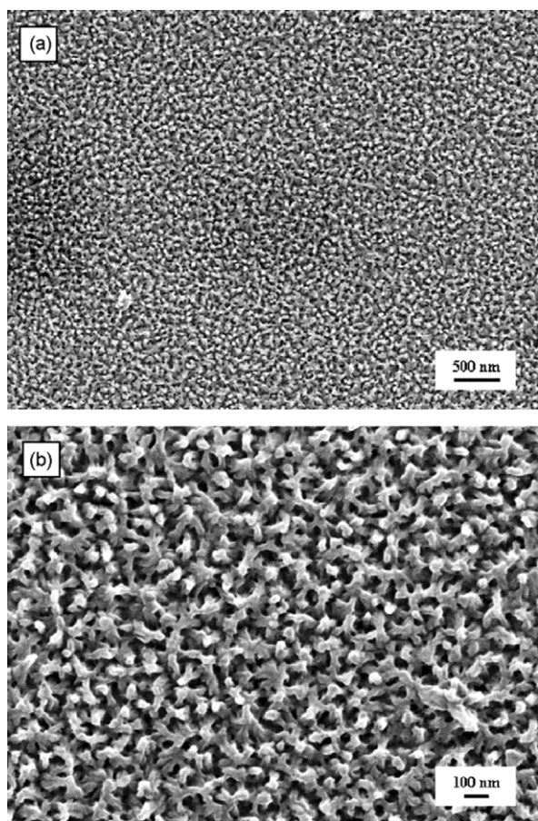
Figure 12. (a) SEM micrograph of a PANi nanofibril mat on an ITO glass electrode, and (b) higher magnification of picture (a). Reprinted from Ref. 53 with permission from Elsevier.
