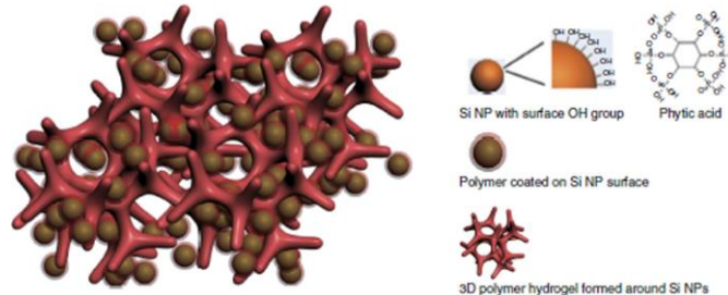
Figure 21. Illustration of the 3D porous Si nano-particles/conductive polymer hydrogel composite electrode. PANi hydrogel framework encapsulate the Si nanoparticles. Si nanoparticles are coated with the PANi layer either through interactions between surface -OH groups and the phosphonic acids in the cross-linker phytic acid molecules (right column), or the electrostatic interaction between negatively charged -OH groups and positively charge PANi due to phytic acid doping. Reprinted by permission from Macmillan Publishers Ltd: Nature Communications 5 , copyright (2013)
