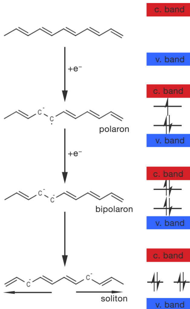
Figure 5. Schematic showing the steps of formation of a polaron, bipolaron and soliton in trans -polyacetylene.
