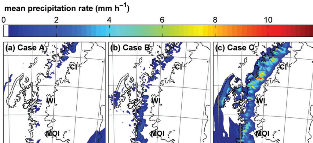
Figure 16. Mean precipitation rate for the 12 h after (a) 2200 UTC on 4 February 2011 during case A, (b) 1200 UTC on 27 January during case B, and (c) 1000 UTC 15 November 2010 during case C, according to the MetUM 1.5 km simulation.
