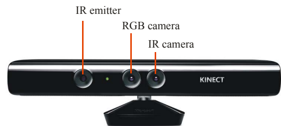
Figure 1. Kinect sensor
