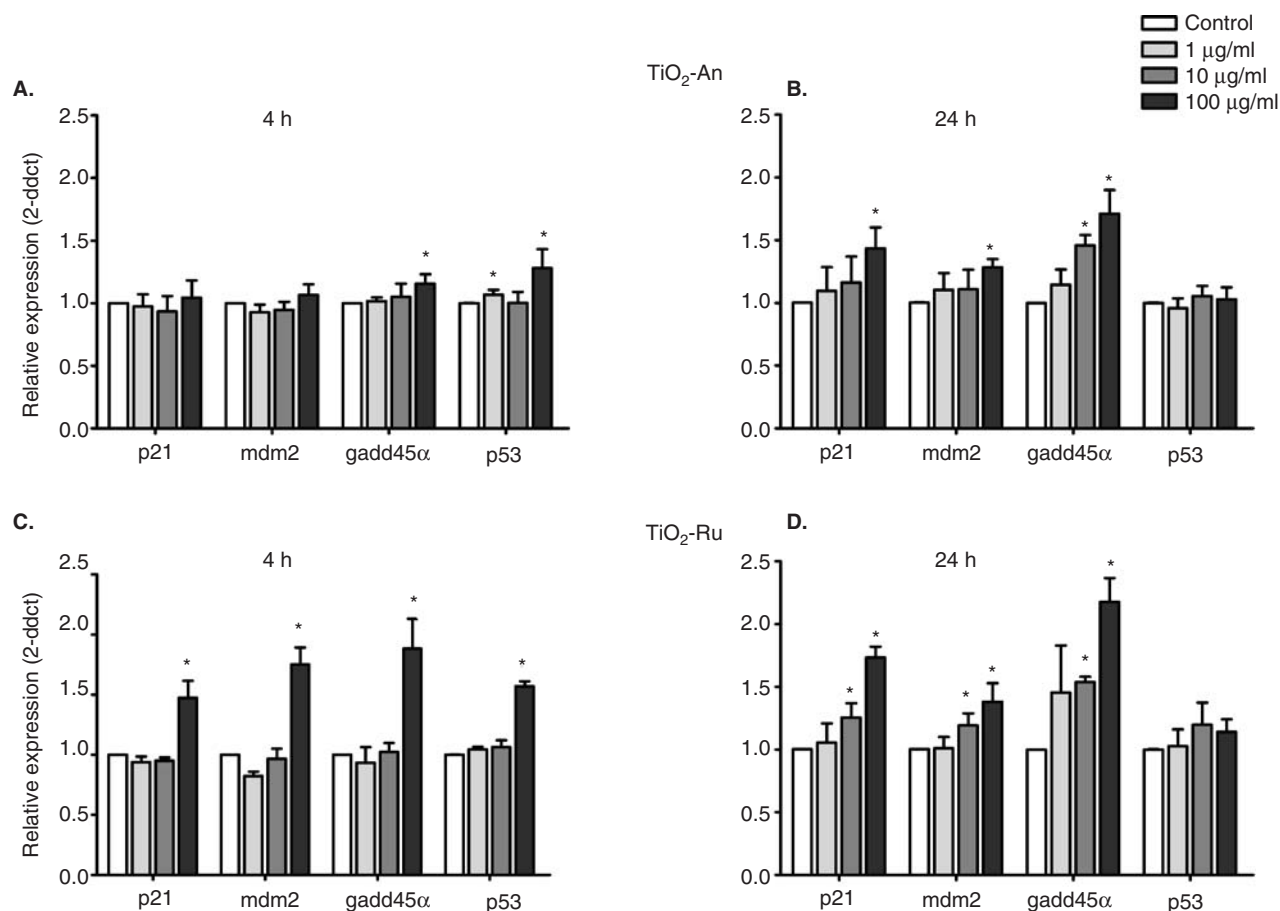
Figure 6. Real-time PCR analysis of the changes in p53 , mdm2 , gadd45 \alpha and p21 gene expression after exposure of HepG2 cells to TiO 2 -An for 4 h (A) and 24 h (B) and TiO 2 -Ru after exposure for 4 h (C) and 24 h (D). The cells were exposed to TiO 2 NPs (0, 1, 10 and 100 \mu g/ml) for 4 and 24 h, then the RT-PCR was performed as described in Materials and methods . The results are expressed as relative mRNA expression normalized to untreated control. Duplicate experiments were repeated at least three times. (*) Denotes a significant difference between TiO 2 NPs-treated groups and control (Student's t -test; P < 0.05).
