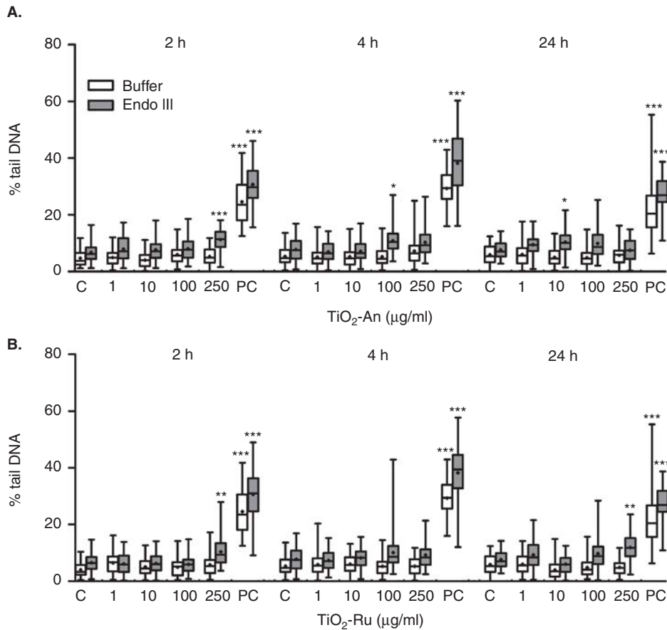
Figure 5. Induction of Endo III-sensitive sites by TiO 2 -An (A) and TiO 2 -Ru (B) in HepG2 cells. The cells were exposed to TiO 2 NPs (0, 1, 10, 100 and 250 µg/ml) for 2, 4 and 24 h, then the modified comet assay was performed as described in Materials and methods . The levels of DNA strand breaks and oxidized pyrimidines are expressed as percent of tail DNA. Fifty cells were analyzed per experimental point in each of the two independent experiments. Data are presented as quantile box plots (for details see the caption of Figure 3). * P < 0.05, ** P < 0.01 and *** P < 0.001 denotes a significant difference between TiO 2 NPs-treated and control groups with and without Endo III, respectively, using ANOVA, Kruskal-Wallis with Dunnet's post test.
