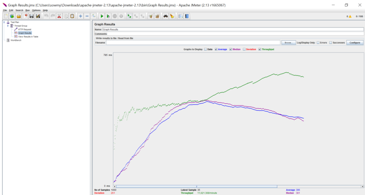
Figure 6.2 Screenshot of graph results of test case 1 in jmeter for 1000 samples.
