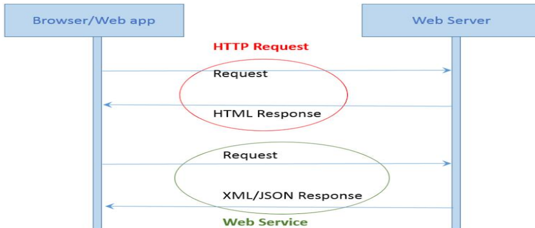
Figure 4.4 Diagram explaining web service request
