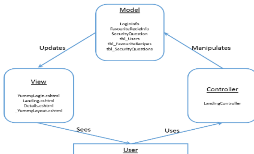
Figure 4.3 MVC architecture of this application
