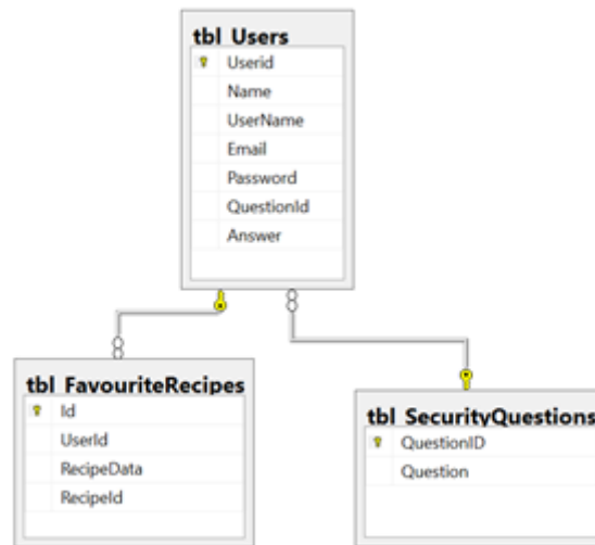
Figure 4.6 Database Diagram of application.
