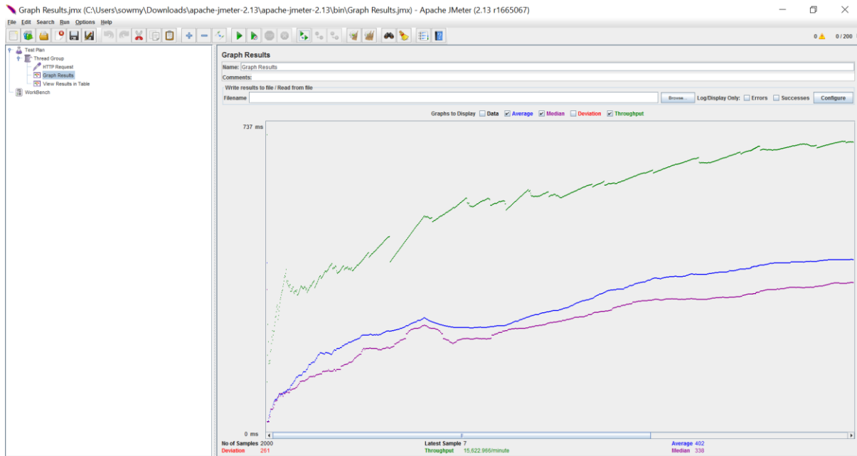
Figure 6.3 Screenshot of graph results of test case 1 in jmeter for 2000 samples.
