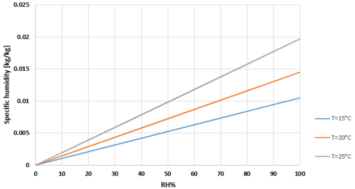
Figure 3: Relationship between relative humidity and specific humidity
