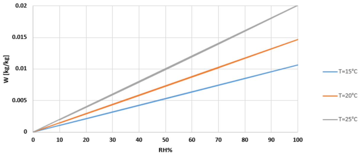
Figure 2: Relationship between relative humidity and humidity ratio
