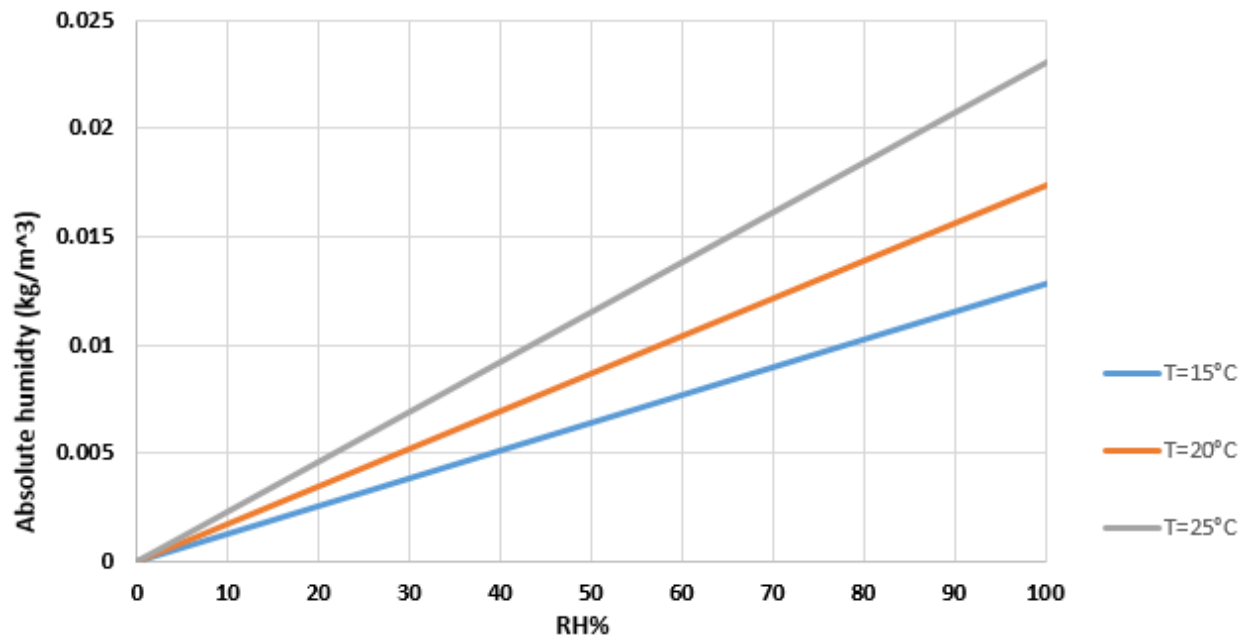
Figure 4: Relationship between relative humidity and absolute humidity
