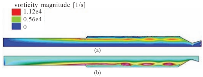
Figure 5. Vorticity plot: (a) for present simulation and (b) for simulation in literature.
