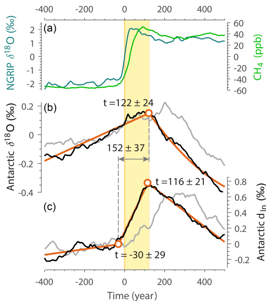
Figure 5. (a) Stack of Greenland NGRIP isotopes and CH 4 for the onsets of GI events listed in Table 1a. (b) Antarctic five-core mean δ 18 O (stack of 5 × 21 warming events). Black curve is the same as “mean” in Fig. 4, centre; grey curve applies the bipolar methane synchronization of WAIS Divide Project Members (2015). (c) Antarctic five-core mean deuterium excess ( d ln ). Black curve is the same as “mean” in Fig. 4e, f; grey curve applies the bipolar methane synchronization of WAIS Divide Project Members (2015). Orange curves are fitting functions using the change-point analysis applied in WAIS Divide Project Members (2015). The stated 2σ uncertainty estimates are obtained from a Monte Carlo sampling (see main text). When the same uncertainty estimate is made for the GI terminations (Fig. 4) the δ 18 O timing is at 101 ± 29 years, the d ln transition onset is at −59 ± 58 years, and the d ln transition end is at 95 ± 34 years; the duration between the d ln onset and the δ 18 O change point is 160 ± 65 years. The earlier d ln onset for the GI termination probably reflects the GI terminations being generally more gradual than the GI onsets.
