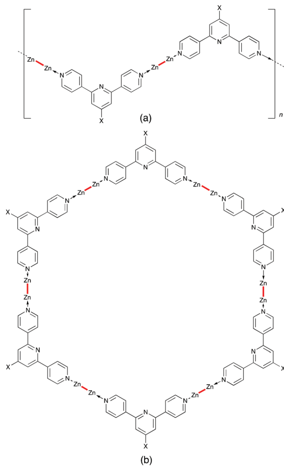
Scheme 5 (a) Schematic representation of a [\text{Zn}_2(\mu\text{-O}_2\text{CR})_4(4'\text{-X-4,2':6',4''}\text{-tpy})]_n polymer ( \text{Zn-Zn} = \text{Zn}_2(\mu\text{-O}_2\text{CR})_4 unit); (b) proposed metallohexacycle (see text).
