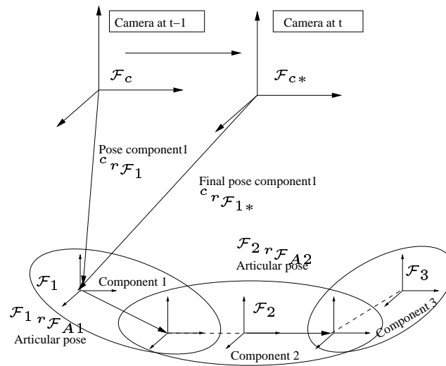
Figure 1: Kinematic chain method: The pose of an articulated object is determined via a kinematic chain of rigid bodies extending to sub components. The poses \mathcal{r} describing the state of the system are intuitive.
