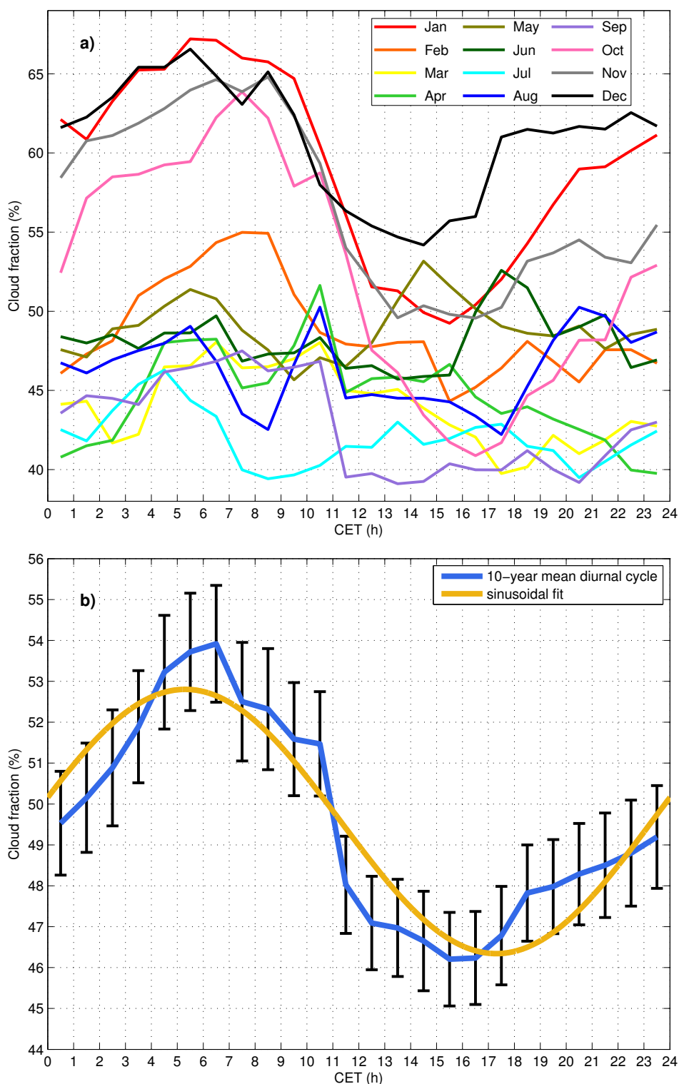
Figure 7. Cloud fraction diurnal cycle measured by TROWARA at Bern. The time on the x-axis is in CET (Central European Time). (a) Cloud fraction diurnal cycle for each month averaged over the 2004–2013 period. (b) Blue line: 10-year mean cloud fraction diurnal cycle (averaged over 120 months) with the black bars showing the standard deviation of the mean for each hour. Yellow line: sinusoidal fit.
