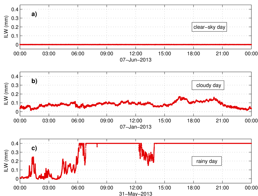
Figure 1. Integrated cloud liquid water (ILW) measured by TROWARA at 3 different situations: (a) on a clear-sky day ( \text{ILW} \sim 0 \text{ mm} ), (b) on a cloudy day ( \text{ILW} > 0 \text{ mm} ) and (c) on a day with precipitation events, during which ILW assumes the maximum allowed value of 0.4 mm.
