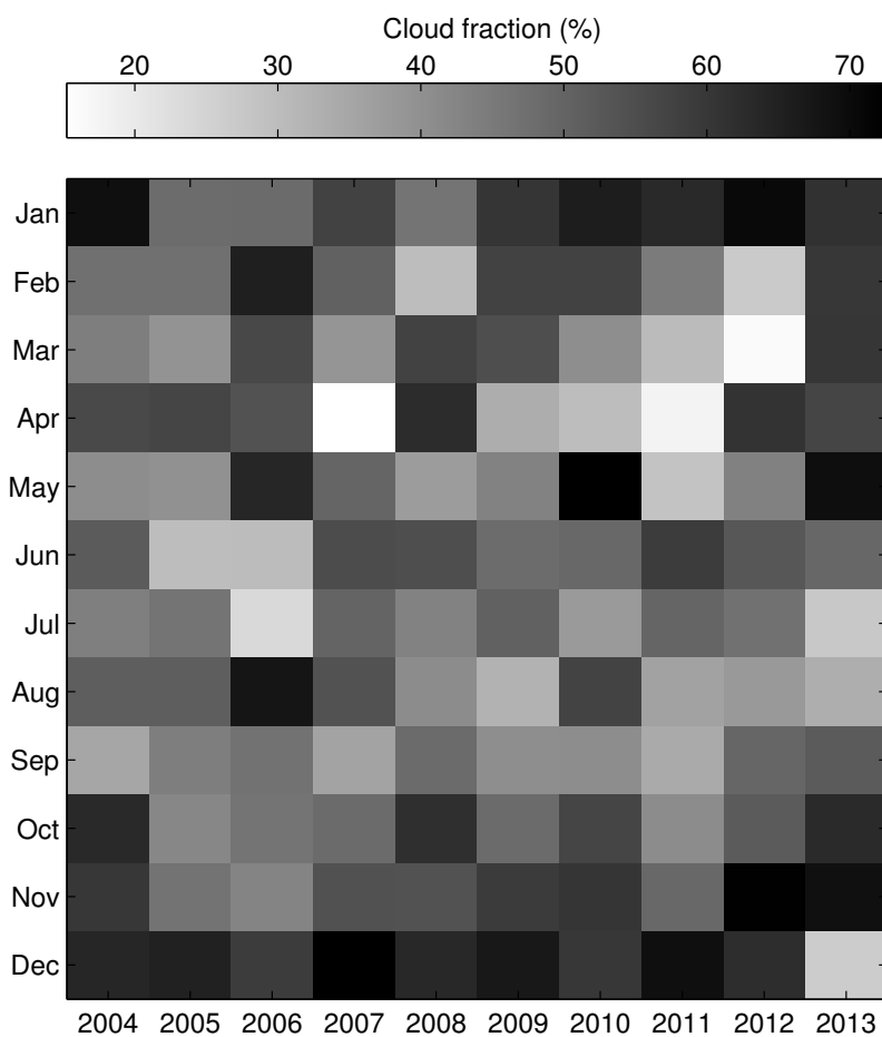
Figure 4. Cloud fraction measured by TROWARA at Bern for every month of the period 2004–2013.
