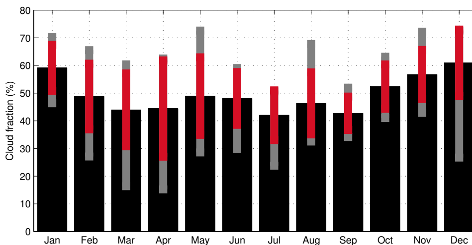
Figure 3. Ten-year cloud fraction (CF) climatology over Bern for the period 2004–2013. The black bars represent the 10-year average CF, the red bars the standard deviation and the grey bars the range between the minimum and maximum values.
