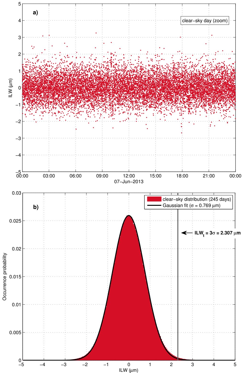
Figure 2. (a) ILW measured by TROWARA on a day without clouds. The ILW values are scattered around zero and usually never exceed \pm 5 \mu\text{m} . (b) Distribution of the ILW values measured by TROWARA in clear-sky conditions (red bars). The sample from which the distribution is computed consists of 245 days in which the sky is free of clouds ( -5 \mu\text{m} < \text{ILW} < 5 \mu\text{m} ), as in (a). The black line is the Gaussian fit of the distribution, which provides the standard deviation of the measurement error around zero ( \sigma = 0.769 \mu\text{m} ). The grey vertical line is the cloudy-sky threshold \text{ILW}_t , which we set equal to 3\sigma . ILW measurements greater than \text{ILW}_t will correspond to cloudy-sky conditions with a confidence level of 99.9%.
