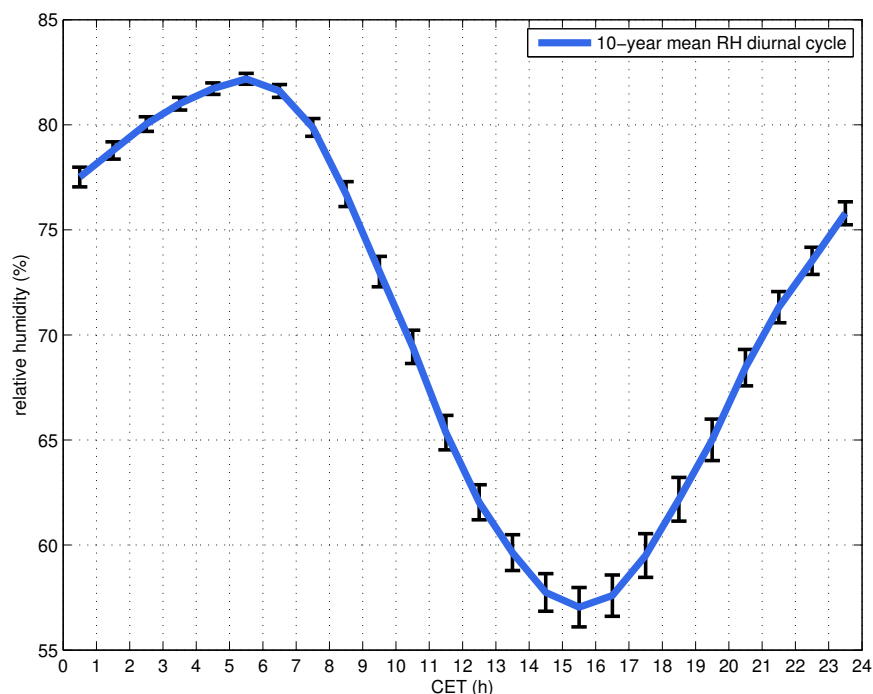
Figure 8. Relative humidity diurnal cycle measured by the local meteorological station at Bern. The time on the x-axis is in CET (Central European Time). The blue line shows the 10-year mean relative humidity diurnal cycle (averaged over 120 months) with the black bars showing the standard deviation of the mean for each hour. The relative humidity diurnal cycle is in phase with the cloud fraction diurnal cycle (Figure 7).
