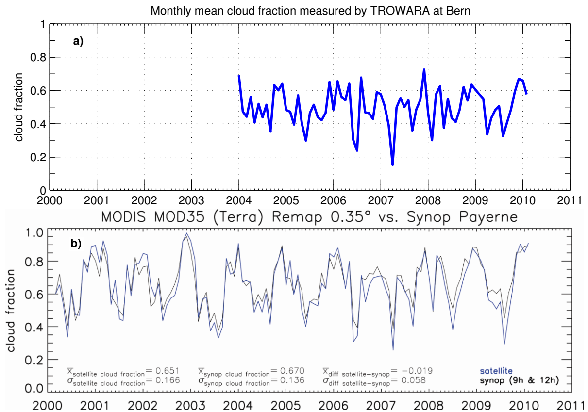
Figure 5. Comparison of monthly mean cloud fraction measured (a) at Bern (46.95° N, 7.44° E) and (b) at Payerne (46.80° N, 6.93° E). (a) Cloud fraction time series measured by TROWARA at Bern, shown only for the overlapping period with Payerne (January 2004–February 2010). (b) Comparison of MODIS Terra (based on MOD35 data, averaged at 0.35° grid) daytime monthly mean cloud fraction product with ground-based Synop observations at Payerne. The monthly Synop Payerne time series are based on synoptic observations made every three hours by a local observer (average of 9 h and 12 h observations). This figure has been taken from Seiz et al. [15] (Figure 3 in their study).
