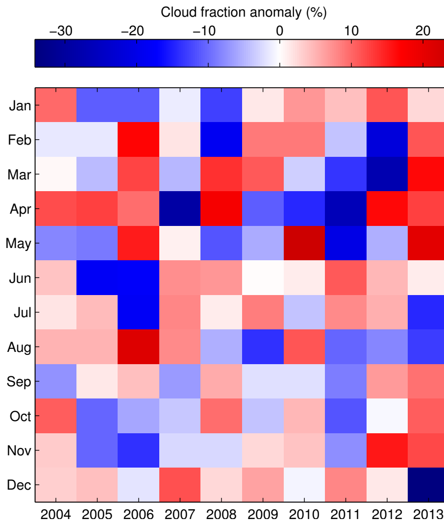
Figure 6. Cloud fraction anomalies compared to the 10-year average values of Table 1.
