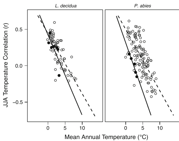
Fig. 6 Pearson correlations for June–August (JJA) temperatures plotted as a function of mean annual temperature for sites across Europe (open circles) and within the Löttschental (filled circles) for both Larix decidua and Picea abies . Trend lines are a linear model fit to European and Löttschental data (dashed and solid, respectively)
