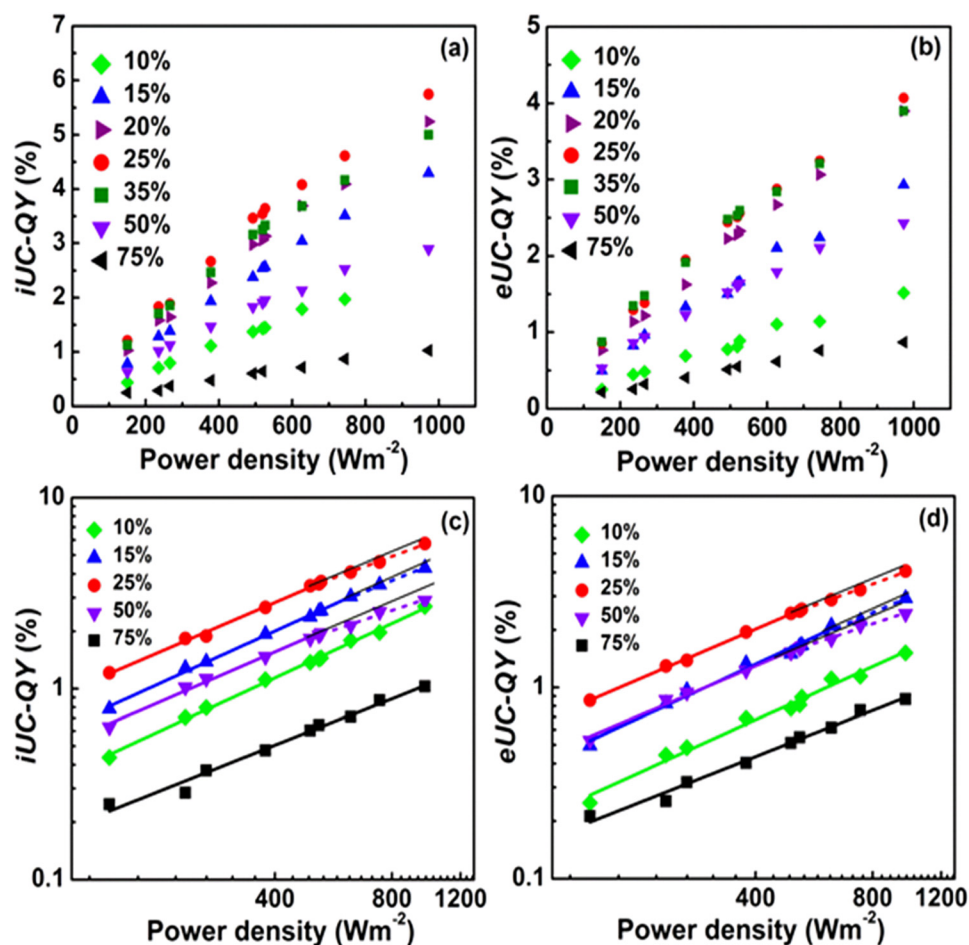
FIG. 3. Variation in the (a) iUC-QY and (b) eUC-QY as a function of excitation power density for different Er^{3+} concentrations. The log-log plots of the (c) internal and (d) external UC-QY versus the power density show deviations from a linear behavior for high power density and high Er^{3+} concentrations. The lines are fits to the low (solid lines) and high (dotted lines) power density ranges, respectively. Note that for clarity, the corresponding error values [ \pm 10\% in the UC-QY and \pm 4.4\% in the power density] have not been included in the figures.
