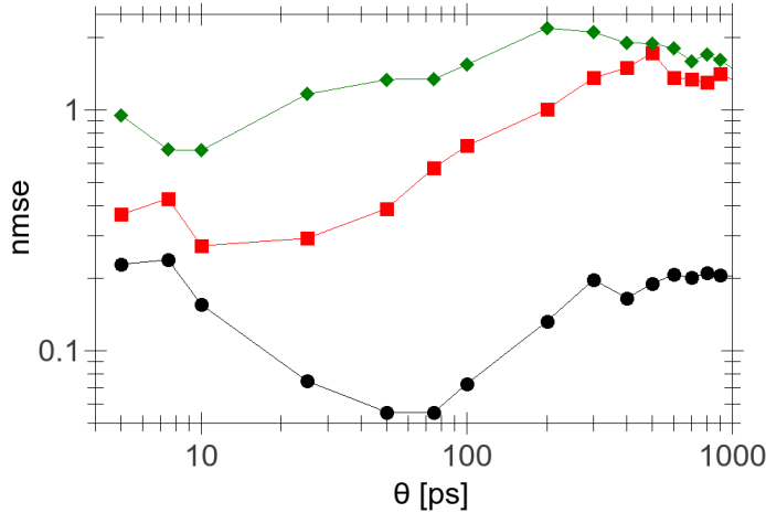
Figure 6.22: NMSE results versus \Theta for different PMOF feedback rates \kappa_{\parallel} = 10 \text{ ns}^{-1} (black circles), \kappa_{\parallel} = 20 \text{ ns}^{-1} (red squares), and \kappa_{\parallel} = 40 \text{ ns}^{-1} (green diamonds). The normalized pump current is p = 1.0 , the other parameters are chosen according to Table 6.1. Note the log-log scale.
