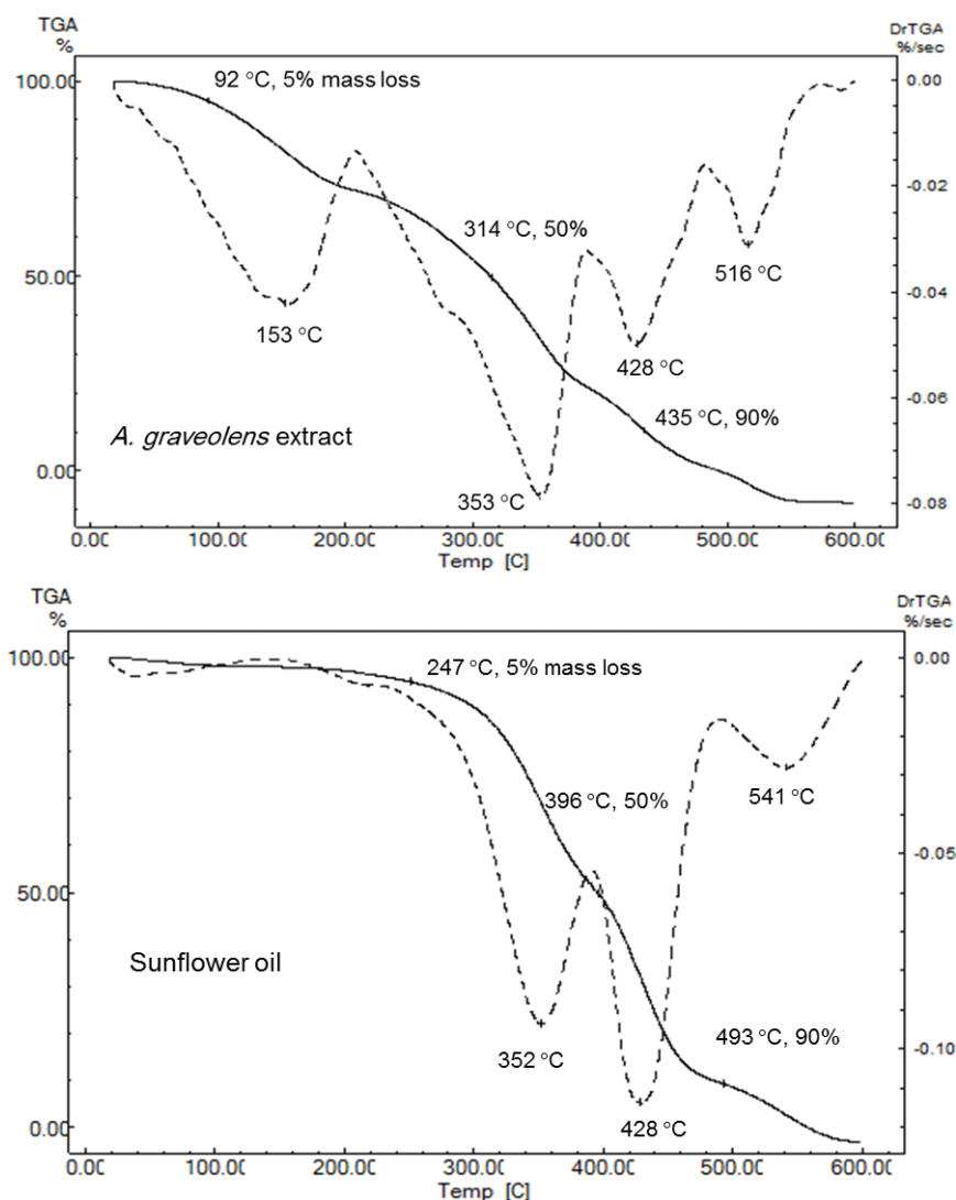
FIGURE 3. Thermogravimetric (TGA) and first derivative thermogravimetric (DTGA) curves of A. graveolens extract and sunflower seed oil.
