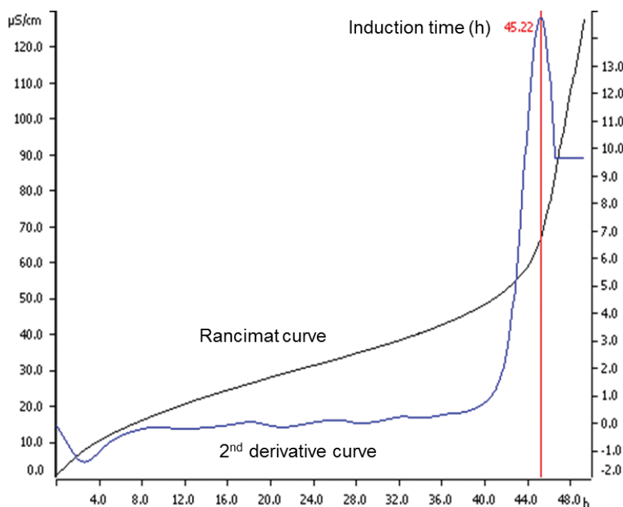
FIGURE 2. Rancimat diagram for A. graveolens seed extract (110 °C).
