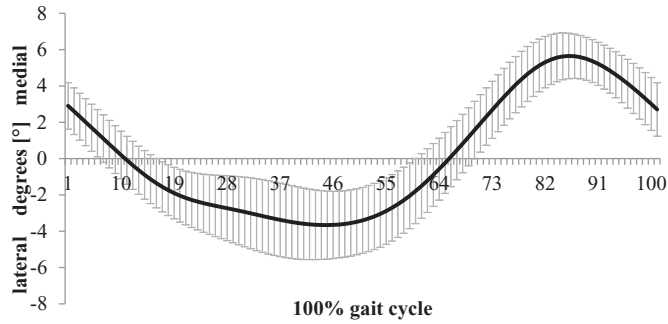
Fig. 2. Kinematic data of lateral trunk bending to the healthy side of one amputee while walking on even ground with variability indicated by the standard deviation. The averaged width standard deviation band constitutes the variability.
