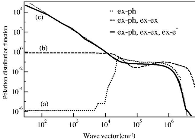
FIG. 2. Distribution function of polaritons at 10 K when non-resonantly pumped with a power of 4.2 \text{ W/cm}^2 . Results are shown for (a) polariton-acoustic phonon scattering (dotted), (b) as (a) plus polariton-polariton scattering (dashed), and (c) as (b) plus polariton-electron scattering (solid). The thin dotted line shows the equilibrium Bose distribution function with zero chemical potential.
