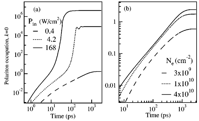
FIG. 3. (a) Polariton occupation of the k=0 state vs time for excitation powers of 0.42 \text{ W/cm}^2 (dashed), 4.2 \text{ W/cm}^2 (dotted), 168 \text{ W/cm}^2 (solid). The pump is turned on at t=0 . The corresponding total polariton equilibrium densities are 7.0 \times 10^8 , 1.3 \times 10^9 , and 1.3 \times 10^{10} \text{ cm}^{-2} . (b) As (a) for a pump power of 0.42 \text{ W/cm}^2 and electron doping of 2.5 \times 10^9 \text{ cm}^{-2} (dashed), 10^{10} \text{ cm}^{-2} (dotted), 4 \times 10^{10} \text{ cm}^{-2} (solid).
