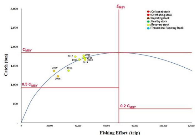
FIGURE 4 Fitted equilibrium Pella & Tomlinson model and fish stock status for Scomberomorus commerson in Banyuasin coastal waters.
