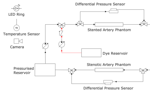
Fig. 3. Schematic of the hydraulic loop
