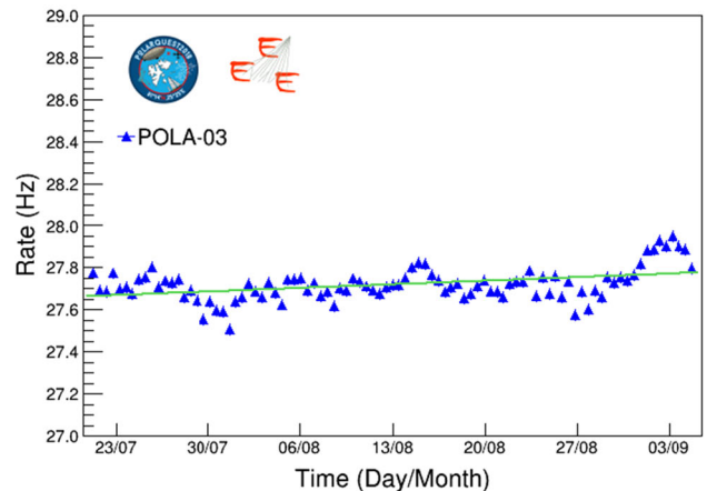
Fig. 27 Cosmic particle rates measured by the POLA detectors as a function of time since July 22, 2018. The green line shows the results of the best fit with a linear function of the time. Note that the scale used for POLA-03 is smaller with respect to the others, to make visible the observed drift
