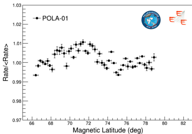
Fig. 26 Top: Rate measured by POLA-01 vs. geographical latitude, divided by the average rate. Bottom: Rate measured by POLA-01 vs. geomagnetic latitude, divided by the average rate
