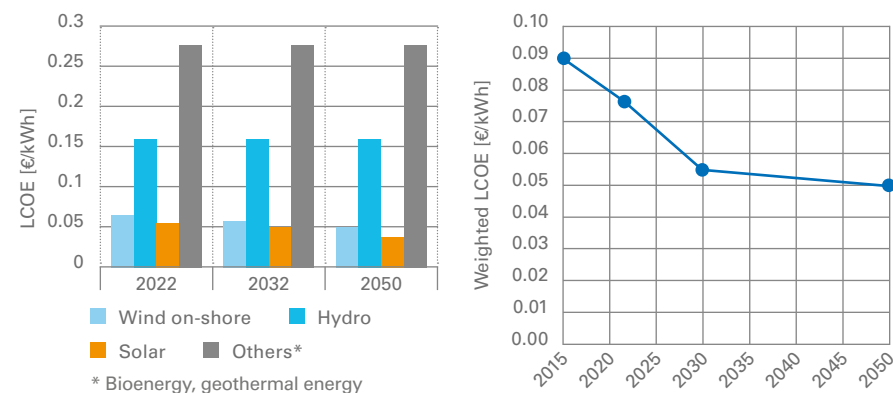
Figure 18 Evolution of LCOE of renewable technologies in Italy.
