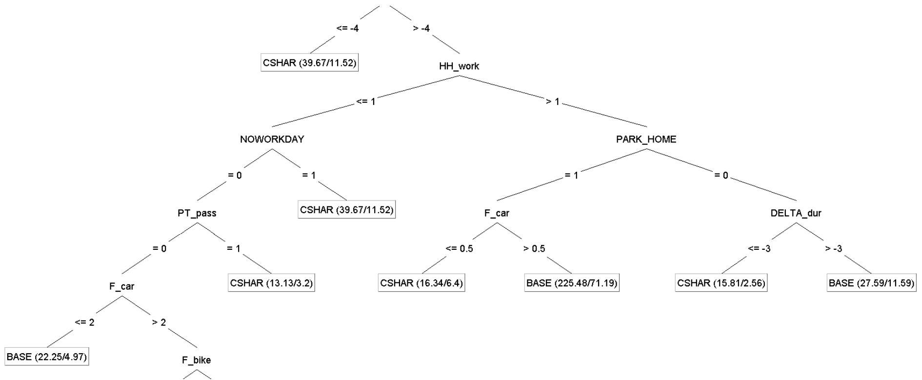
Figure 59. Subfigure II of the decision tree for the switching intentions from car to car sharing (relative values of trip attributes) (
