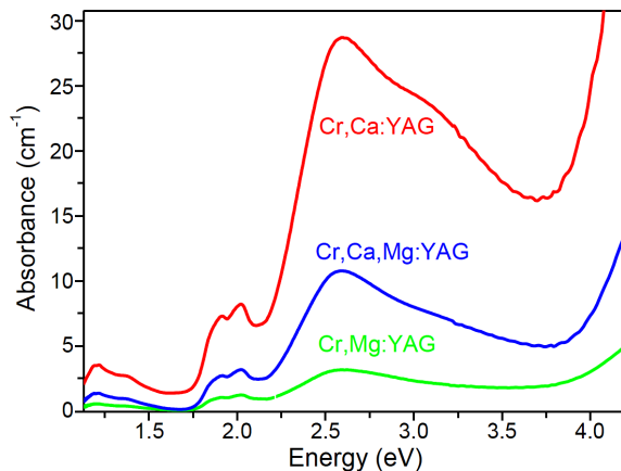
Figure 5. Absorption spectra of \text{Cr}^{4+} in Cr,Ca:YAG (red line), Cr,Ca,Mg:YAG (blue line) and Cr,Mg:YAG (green line) ceramics after vacuum sintering and oxidation annealing
