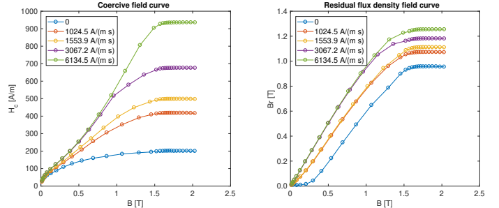
Fig. 4. Coercive field curves (left) and residual flux density curves (right) for the ARMCO® sample as a function of the initial magnetic flux density in the material cross-section, measured at different ramp rates (values at R = 0 retrieved by extrapolation).
